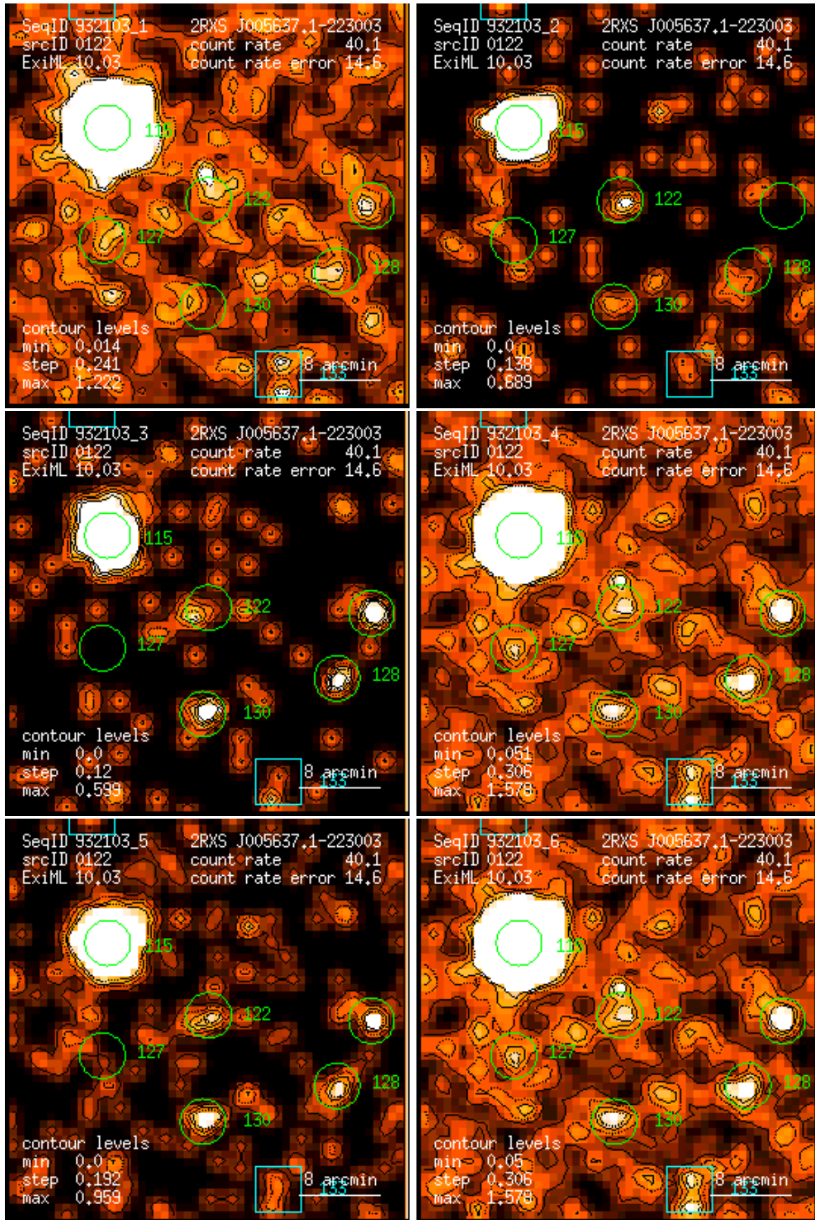
Figure 122: RASS 932103: detection 0122: band rate images, Gaussian filter: (1) PSPC channels 11 – 41, (2) 52 – 90, (3) 91 – 201, (4) 11 – 235, (5) 52 – 201, (6) 11 – 201. Broad band rates in counts/ks. Band rate contour levels in counts/ks/arcmin 2 .
