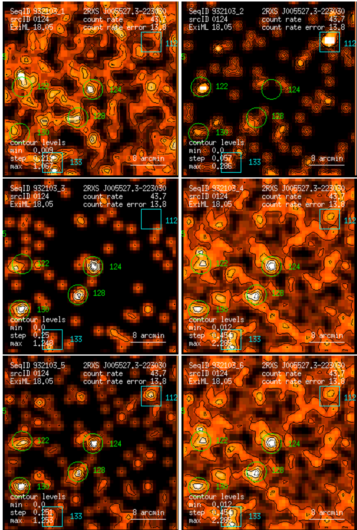
Figure 124: RASS 932103: detection 0124: band rate images, Gaussian filter: (1) PSPC channels 11 – 41, (2) 52 – 90, (3) 91 – 201, (4) 11 – 235, (5) 52 – 201, (6) 11 – 201. Broad band rates in counts/ks. Band rate contour levels in counts/ks/arcmin 2 .
