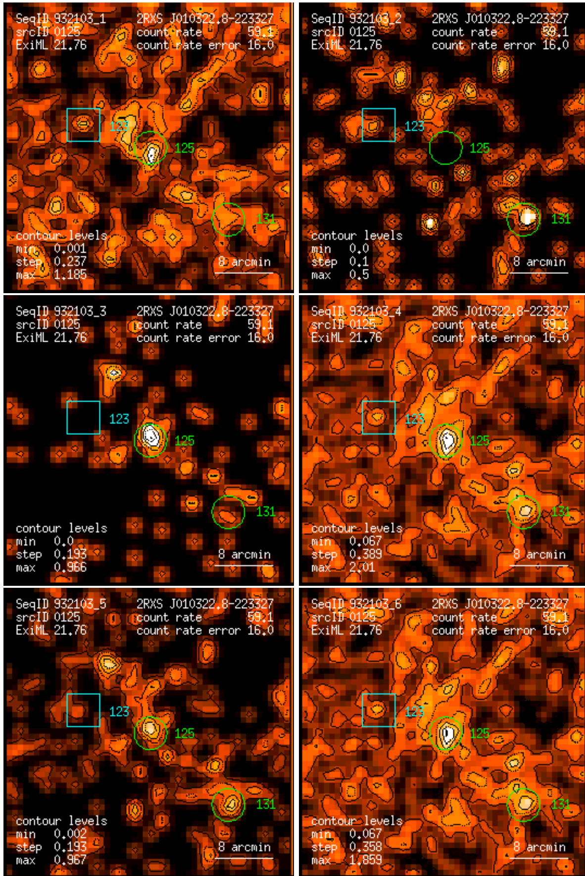
Figure 125: RASS 932103: detection 0125: band rate images, Gaussian filter: (1) PSPC channels 11 – 41, (2) 52 – 90, (3) 91 – 201, (4) 11 – 235, (5) 52 – 201, (6) 11 – 201. Broad band rates in counts/ks. Band rate contour levels in counts/ks/arcmin 2 .
