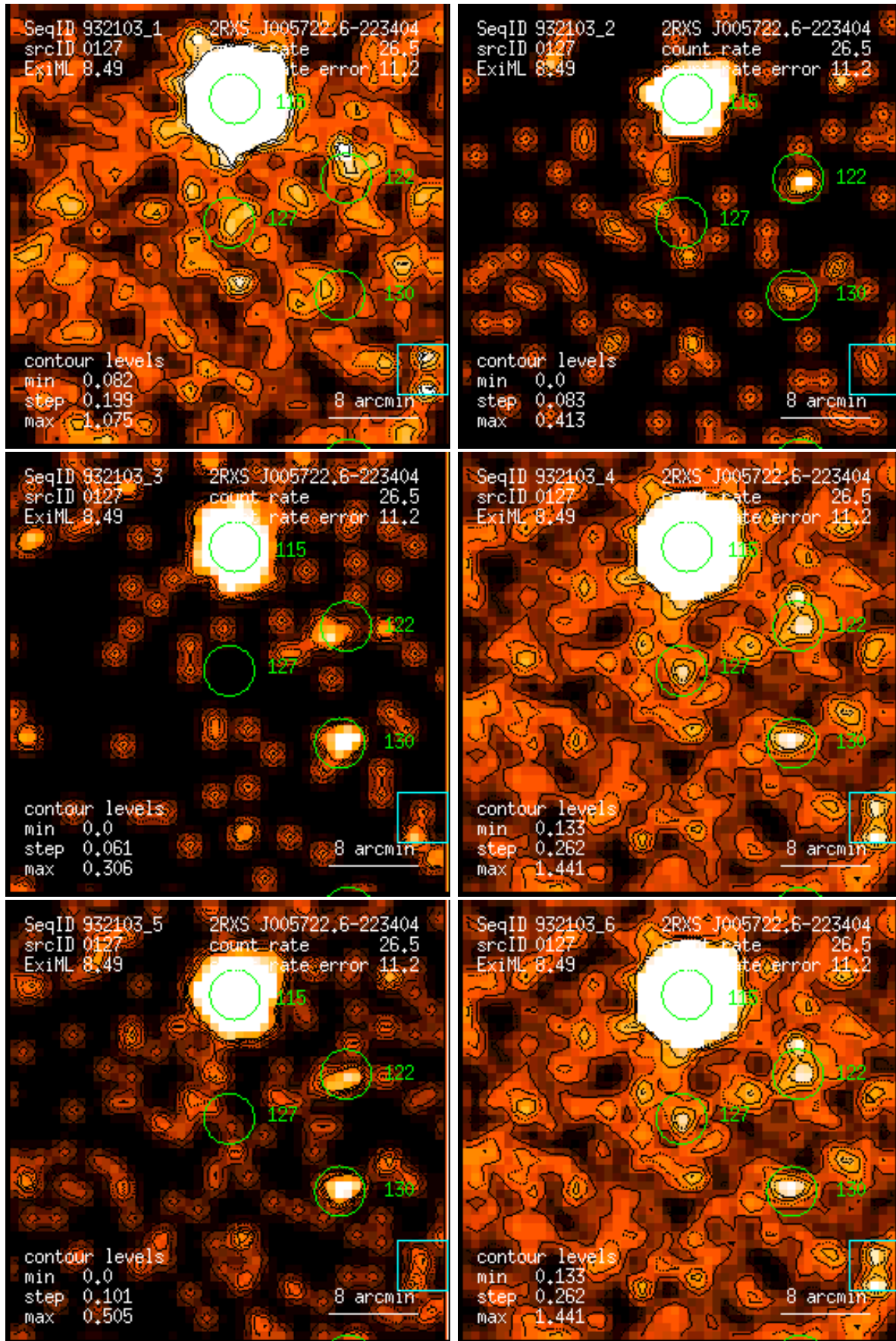
Figure 127: RASS 932103: detection 0127: band rate images, Gaussian filter: (1) PSPC channels 11 – 41, (2) 52 – 90, (3) 91 – 201, (4) 11 – 235, (5) 52 – 201, (6) 11 – 201. Broad band rates in counts/ks. Band rate contour levels in counts/ks/arcmin 2 .
