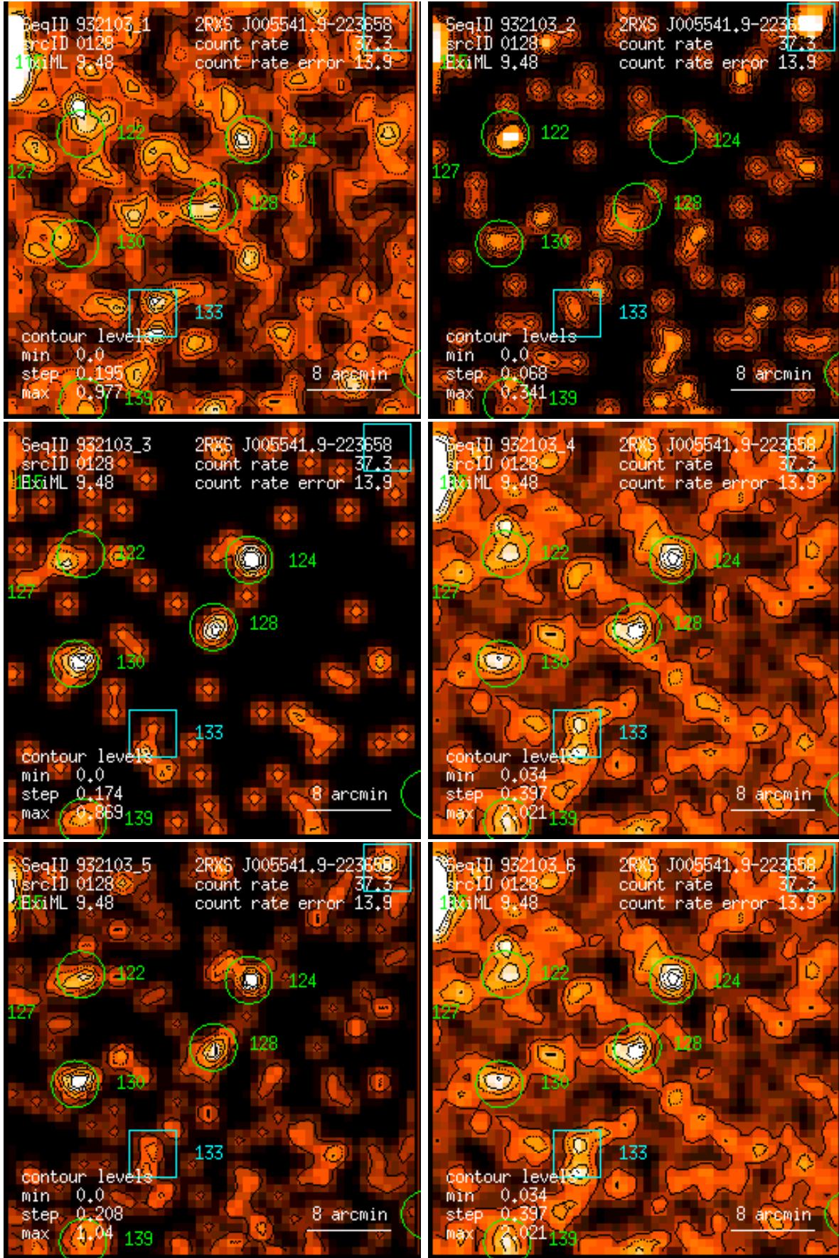
Figure 128: RASS 932103: detection 0128: band rate images, Gaussian filter: (1) PSPC channels 11 – 41, (2) 52 – 90, (3) 91 – 201, (4) 11 – 235, (5) 52 – 201, (6) 11 – 201. Broad band rates in counts/ks. Band rate contour levels in counts/ks/arcmin 2 .
