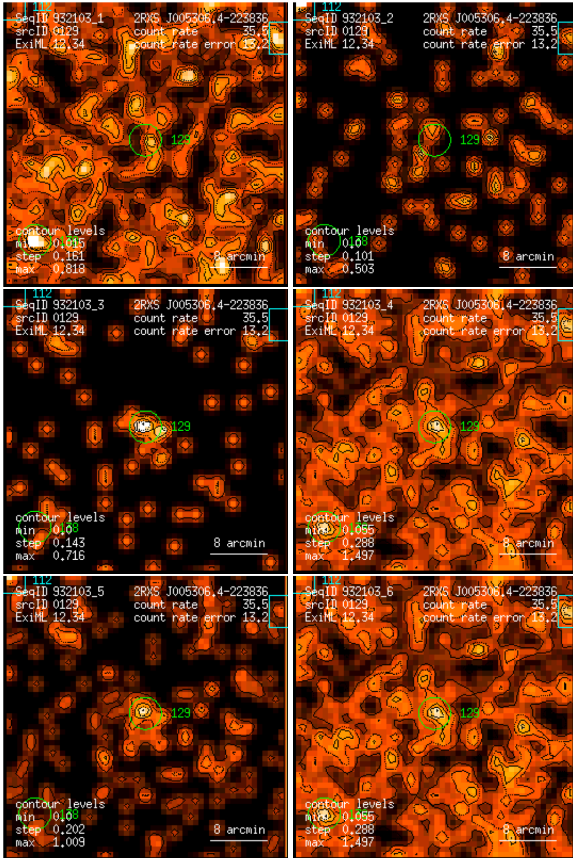
Figure 129: RASS 932103: detection 0129: band rate images, Gaussian filter: (1) PSPC channels 11 – 41, (2) 52 – 90, (3) 91 – 201, (4) 11 – 235, (5) 52 – 201, (6) 11 – 201. Broad band rates in counts/ks. Band rate contour levels in counts/ks/arcmin 2 .
