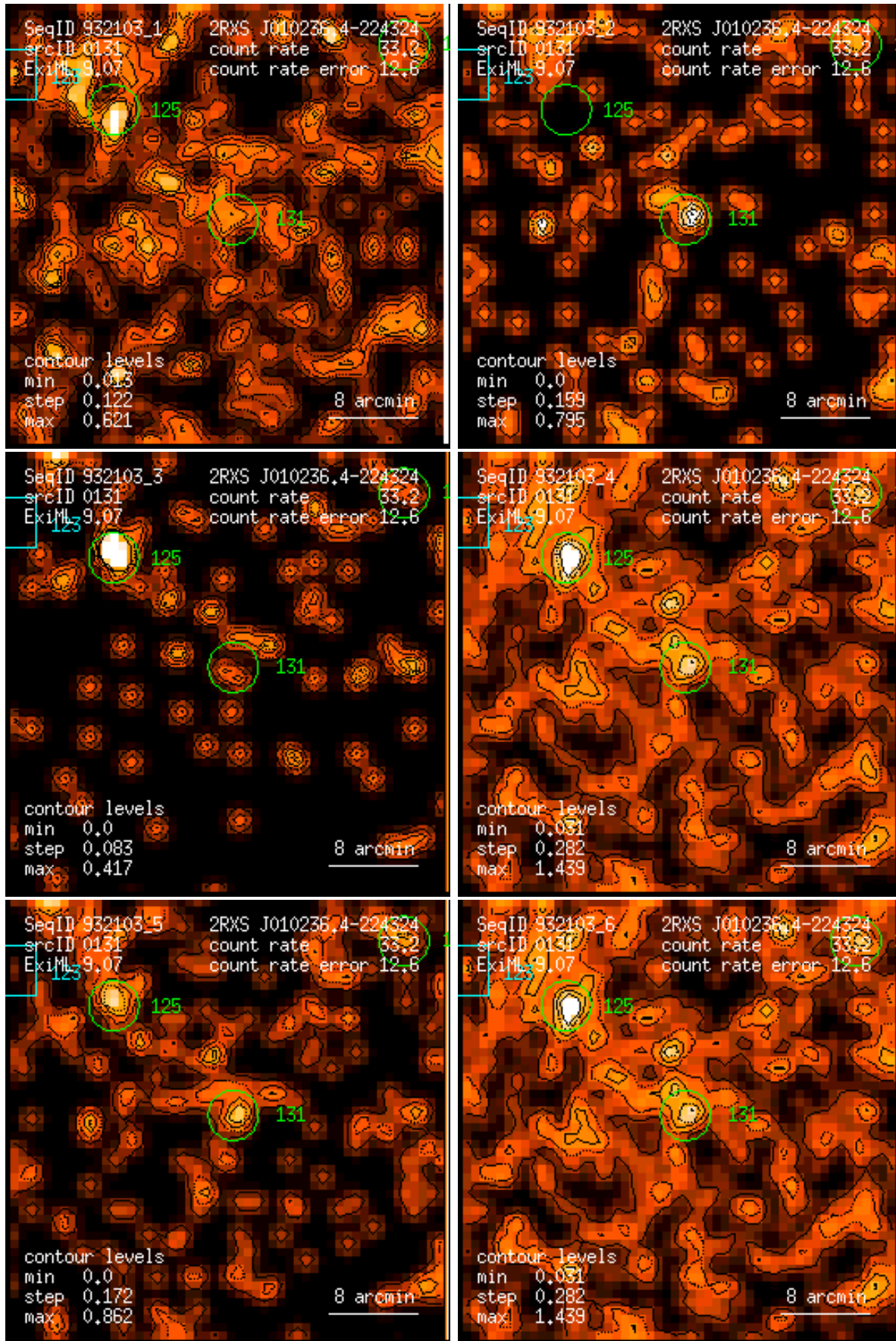
Figure 131: RASS 932103: detection 0131: band rate images, Gaussian filter: (1) PSPC channels 11 – 41, (2) 52 – 90, (3) 91 – 201, (4) 11 – 235, (5) 52 – 201, (6) 11 – 201. Broad band rates in counts/ks. Band rate contour levels in counts/ks/arcmin 2 .
