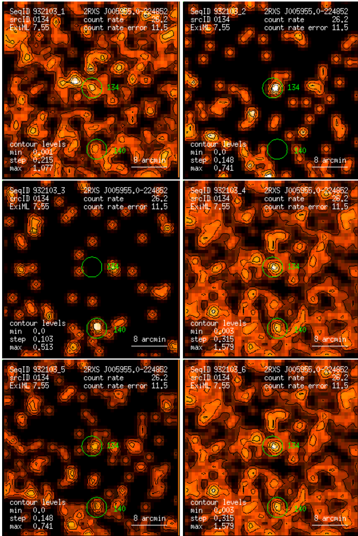
Figure 134: RASS 932103: detection 0134: band rate images, Gaussian filter: (1) PSPC channels 11 – 41, (2) 52 – 90, (3) 91 – 201, (4) 11 – 235, (5) 52 – 201, (6) 11 – 201. Broad band rates in counts/ks. Band rate contour levels in counts/ks/arcmin 2 .
