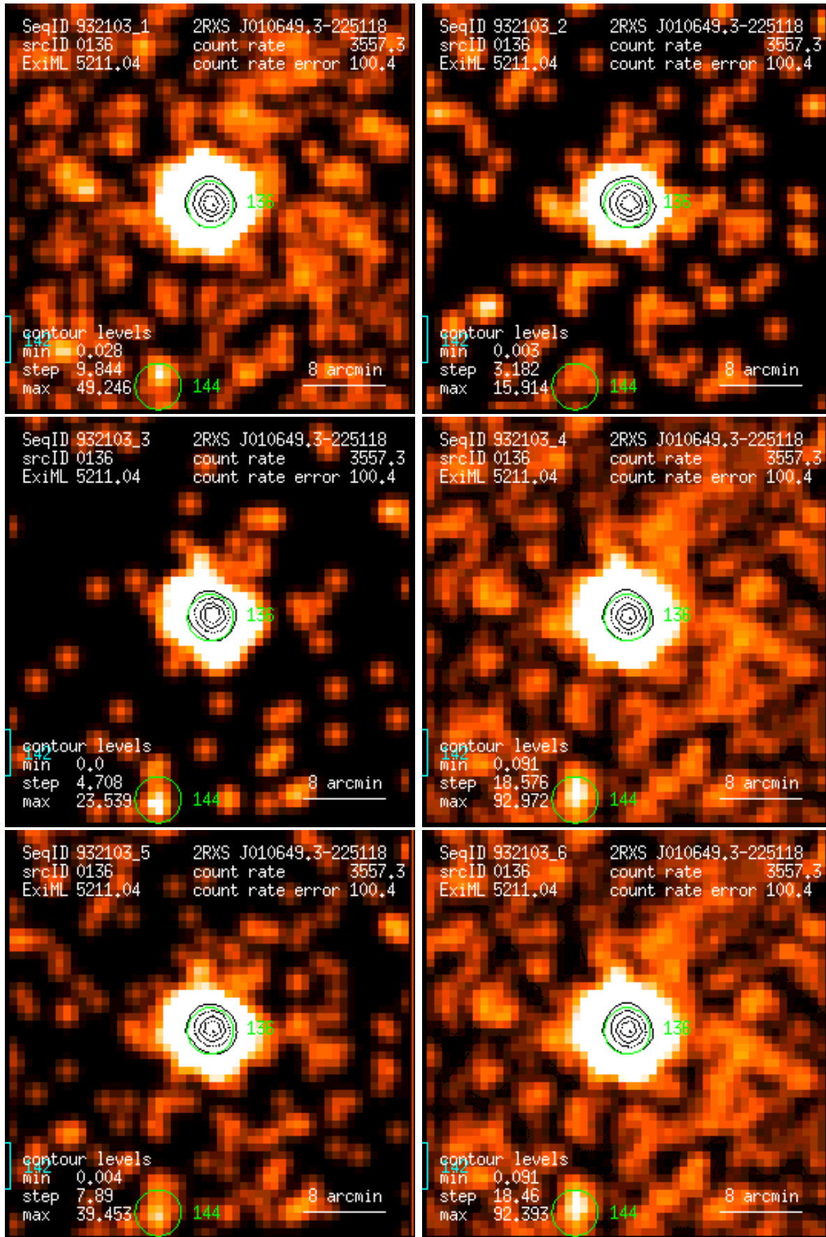
Figure 136: RASS 932103: detection 0136: band rate images, Gaussian filter: (1) PSPC channels 11 – 41, (2) 52 – 90, (3) 91 – 201, (4) 11 – 235, (5) 52 – 201, (6) 11 – 201. Broad band rates in counts/ks. Band rate contour levels in counts/ks/arcmin 2 .
