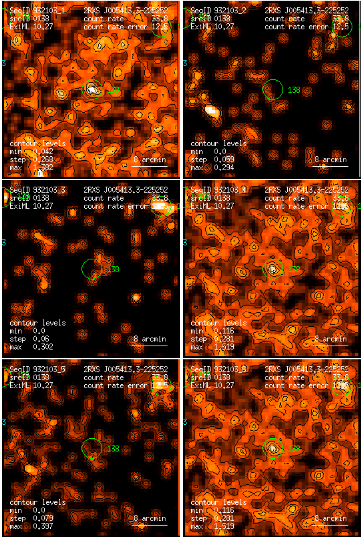
Figure 138: RASS 932103: detection 0138: band rate images, Gaussian filter: (1) PSPC channels 11 – 41, (2) 52 – 90, (3) 91 – 201, (4) 11 – 235, (5) 52 – 201, (6) 11 – 201. Broad band rates in counts/ks. Band rate contour levels in counts/ks/arcmin 2 .
