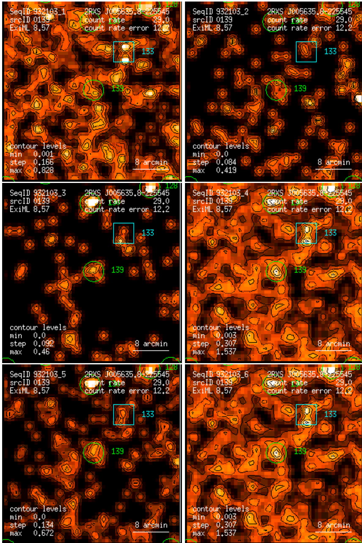
Figure 139: RASS 932103: detection 0139: band rate images, Gaussian filter: (1) PSPC channels 11 – 41, (2) 52 – 90, (3) 91 – 201, (4) 11 – 235, (5) 52 – 201, (6) 11 – 201. Broad band rates in counts/ks. Band rate contour levels in counts/ks/arcmin 2 .
