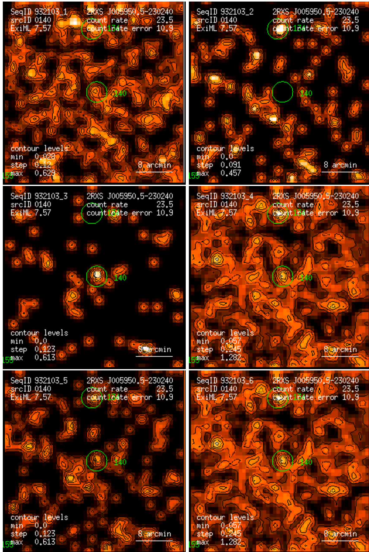
Figure 140: RASS 932103: detection 0140: band rate images, Gaussian filter: (1) PSPC channels 11 – 41, (2) 52 – 90, (3) 91 – 201, (4) 11 – 235, (5) 52 – 201, (6) 11 – 201. Broad band rates in counts/ks. Band rate contour levels in counts/ks/arcmin 2 .
