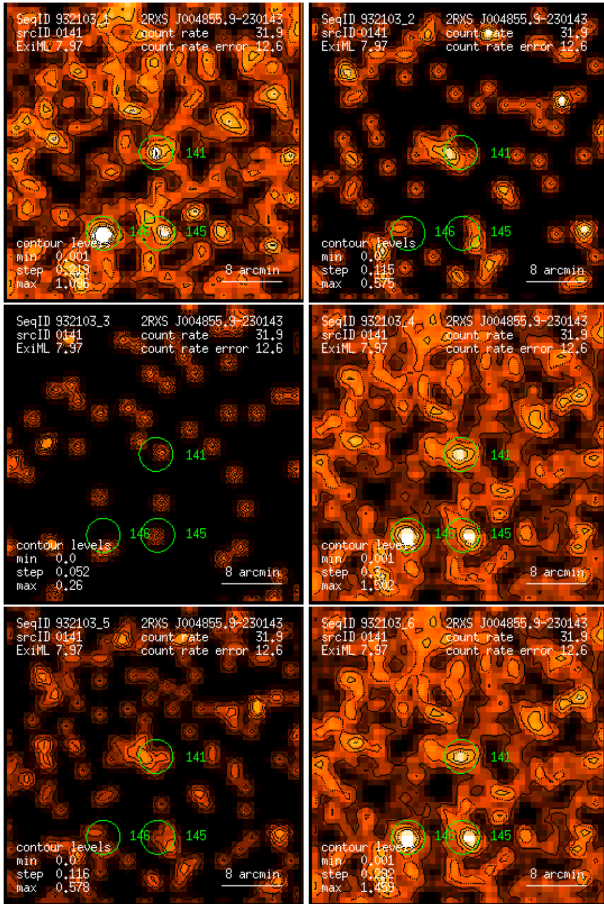
Figure 141: RASS 932103: detection 0141: band rate images, Gaussian filter: (1) PSPC channels 11 – 41, (2) 52 – 90, (3) 91 – 201, (4) 11 – 235, (5) 52 – 201, (6) 11 – 201. Broad band rates in counts/ks. Band rate contour levels in counts/ks/arcmin 2 .
