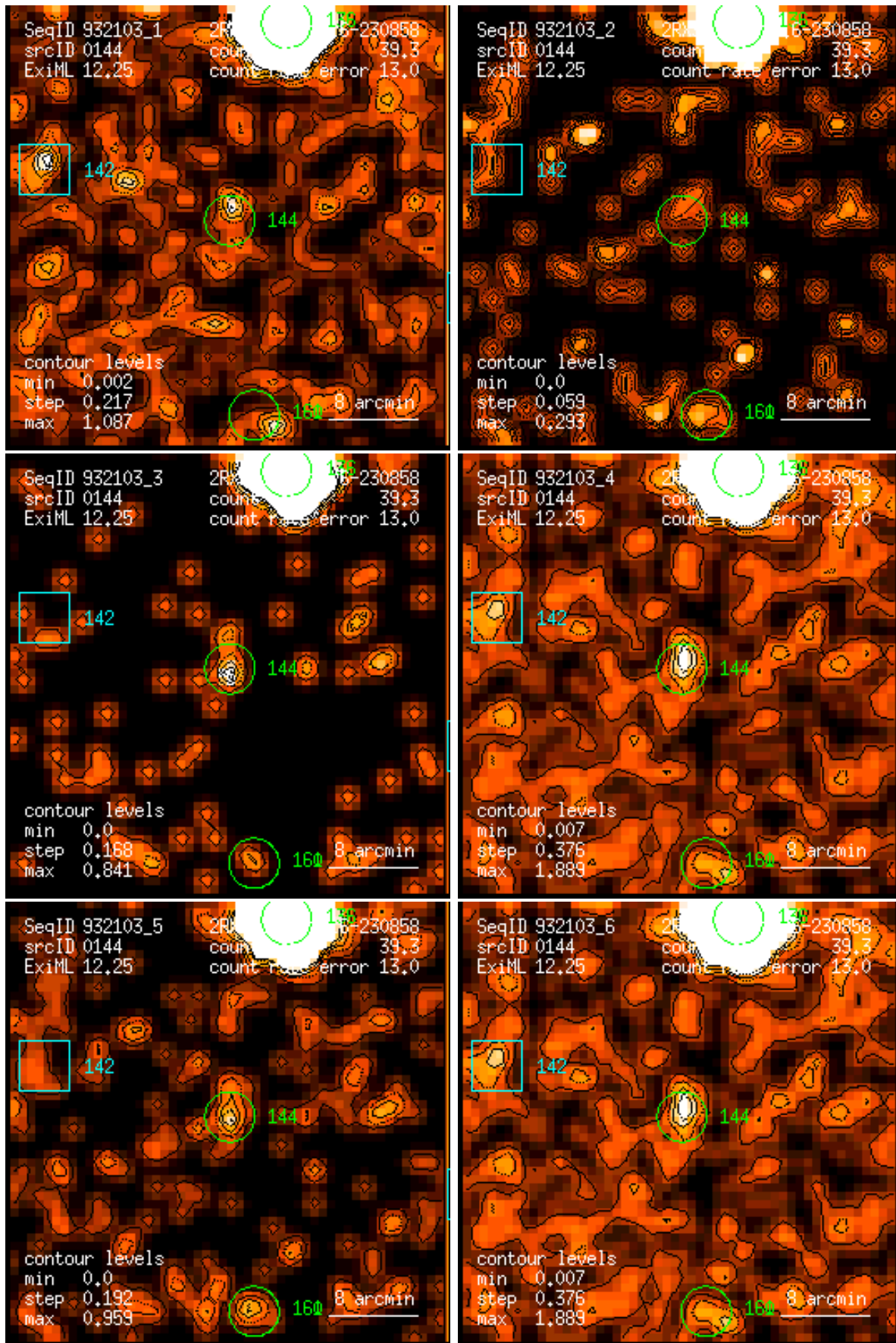
Figure 144: RASS 932103: detection 0144: band rate images, Gaussian filter: (1) PSPC channels 11 – 41, (2) 52 – 90, (3) 91 – 201, (4) 11 – 235, (5) 52 – 201, (6) 11 – 201. Broad band rates in counts/ks. Band rate contour levels in counts/ks/arcmin 2 .
