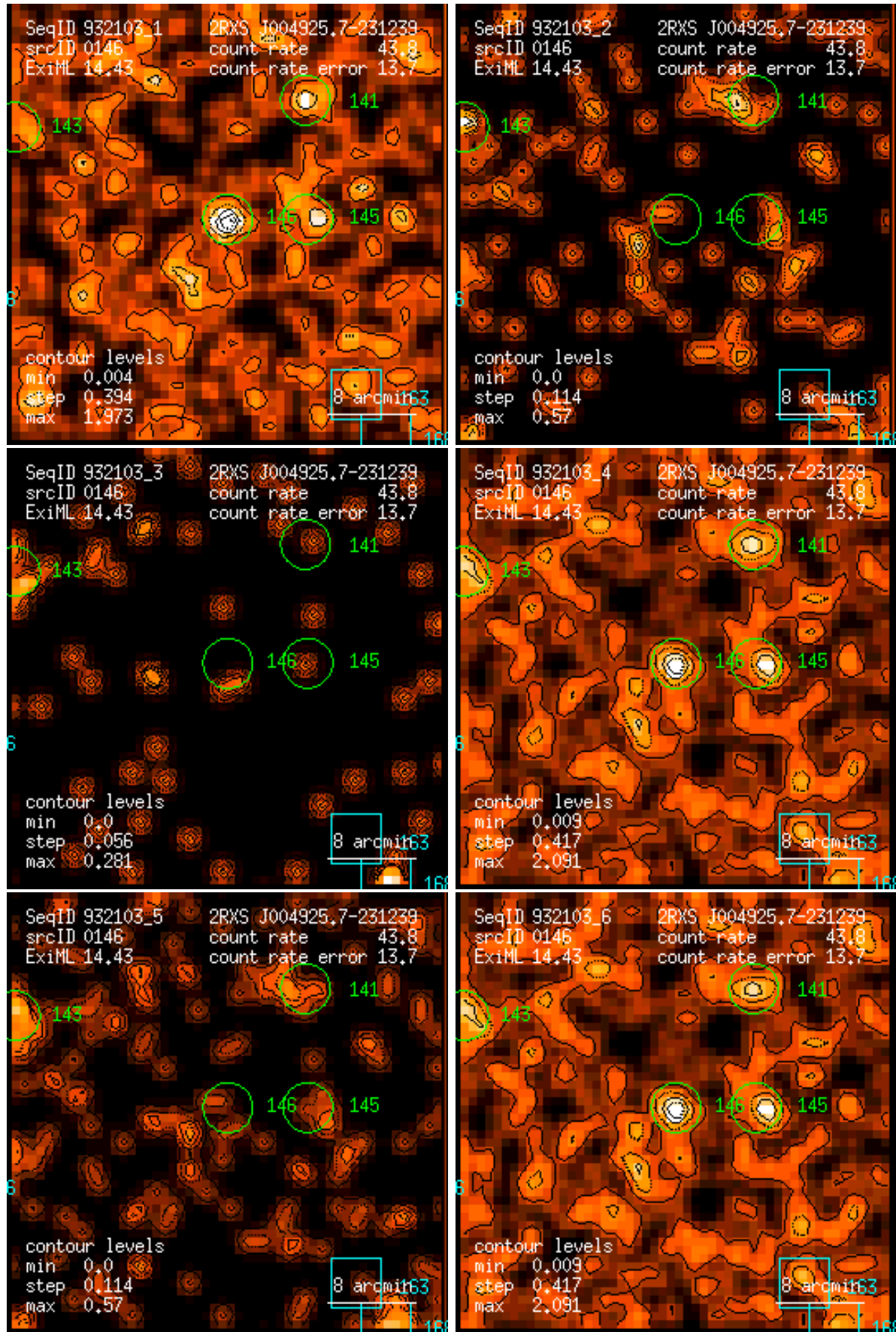
Figure 146: RASS 932103: detection 0146: band rate images, Gaussian filter: (1) PSPC channels 11 – 41, (2) 52 – 90, (3) 91 – 201, (4) 11 – 235, (5) 52 – 201, (6) 11 – 201. Broad band rates in counts/ks. Band rate contour levels in counts/ks/arcmin 2 .
