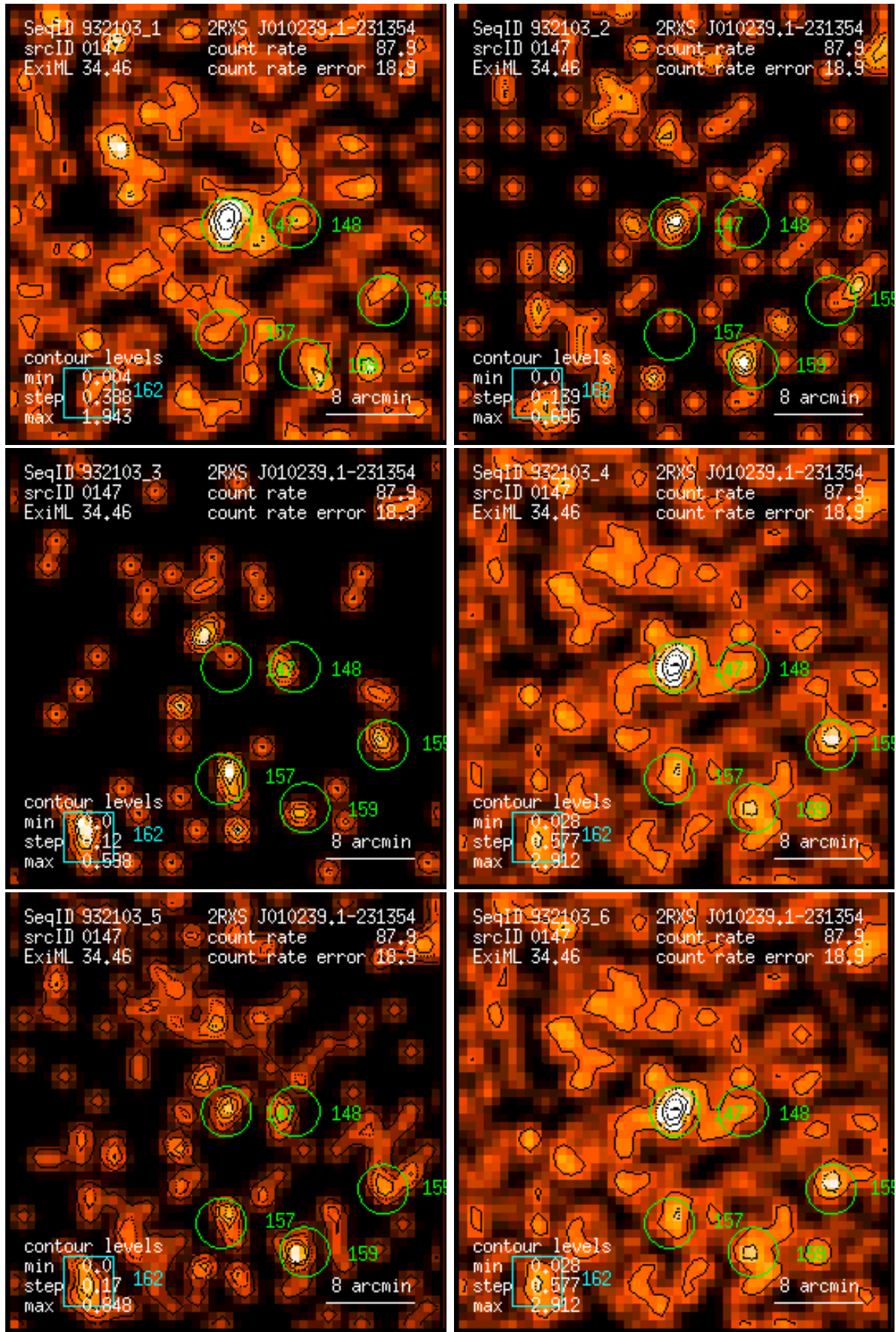
Figure 147: RASS 932103: detection 0147: band rate images, Gaussian filter: (1) PSPC channels 11 – 41, (2) 52 – 90, (3) 91 – 201, (4) 11 – 235, (5) 52 – 201, (6) 11 – 201. Broad band rates in counts/ks. Band rate contour levels in counts/ks/arcmin 2 .
