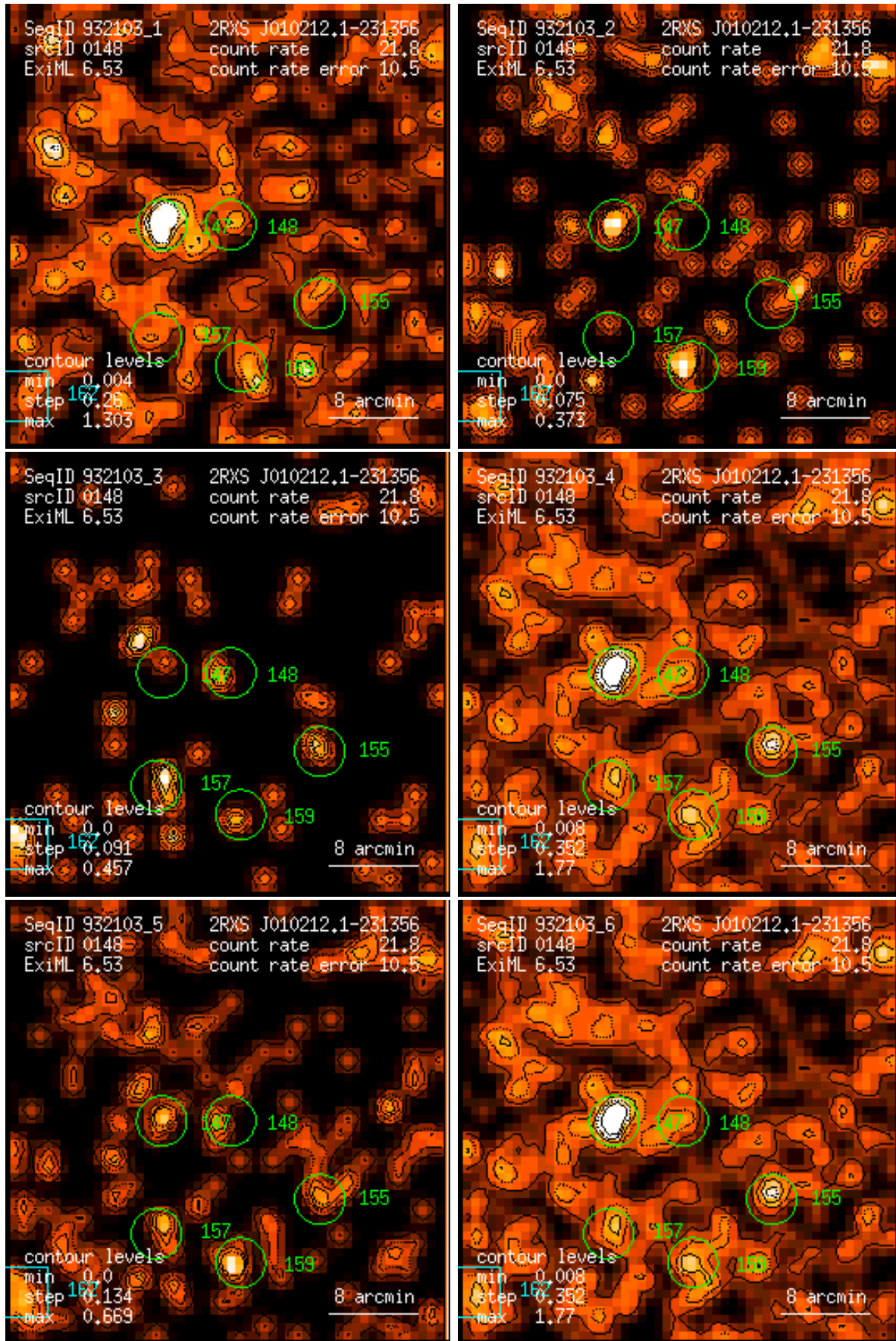
Figure 148: RASS 932103: detection 0148: band rate images, Gaussian filter: (1) PSPC channels 11 – 41, (2) 52 – 90, (3) 91 – 201, (4) 11 – 235, (5) 52 – 201, (6) 11 – 201. Broad band rates in counts/ks. Band rate contour levels in counts/ks/arcmin 2 .
