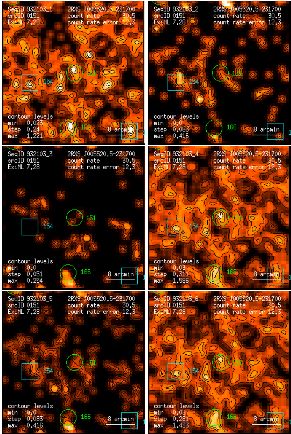
Figure 151: RASS 932103: detection 0151: band rate images, Gaussian filter: (1) PSPC channels 11 – 41, (2) 52 – 90, (3) 91 – 201, (4) 11 – 235, (5) 52 – 201, (6) 11 – 201. Broad band rates in counts/ks. Band rate contour levels in counts/ks/arcmin 2 .
