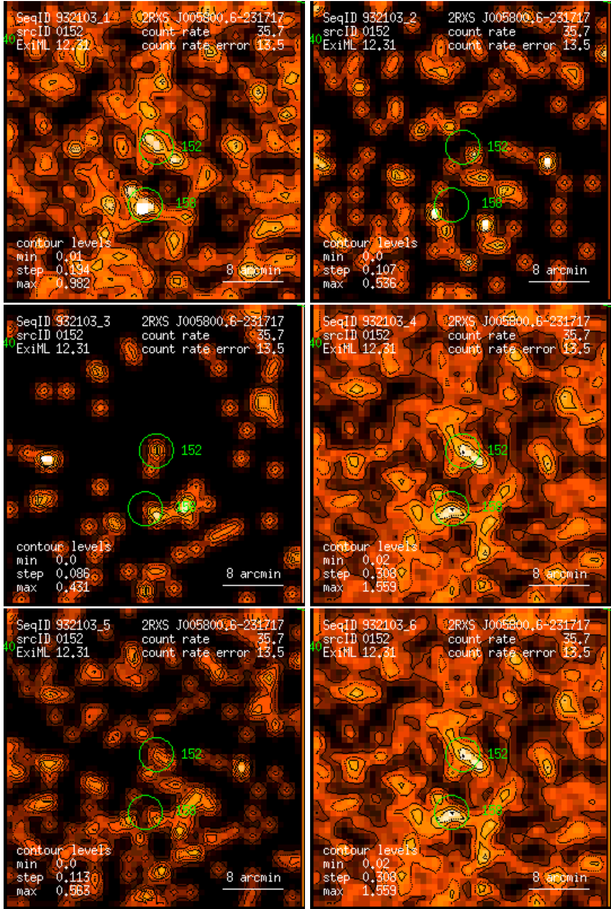
Figure 152: RASS 932103: detection 0152: band rate images, Gaussian filter: (1) PSPC channels 11 – 41, (2) 52 – 90, (3) 91 – 201, (4) 11 – 235, (5) 52 – 201, (6) 11 – 201. Broad band rates in counts/ks. Band rate contour levels in counts/ks/arcmin 2 .
