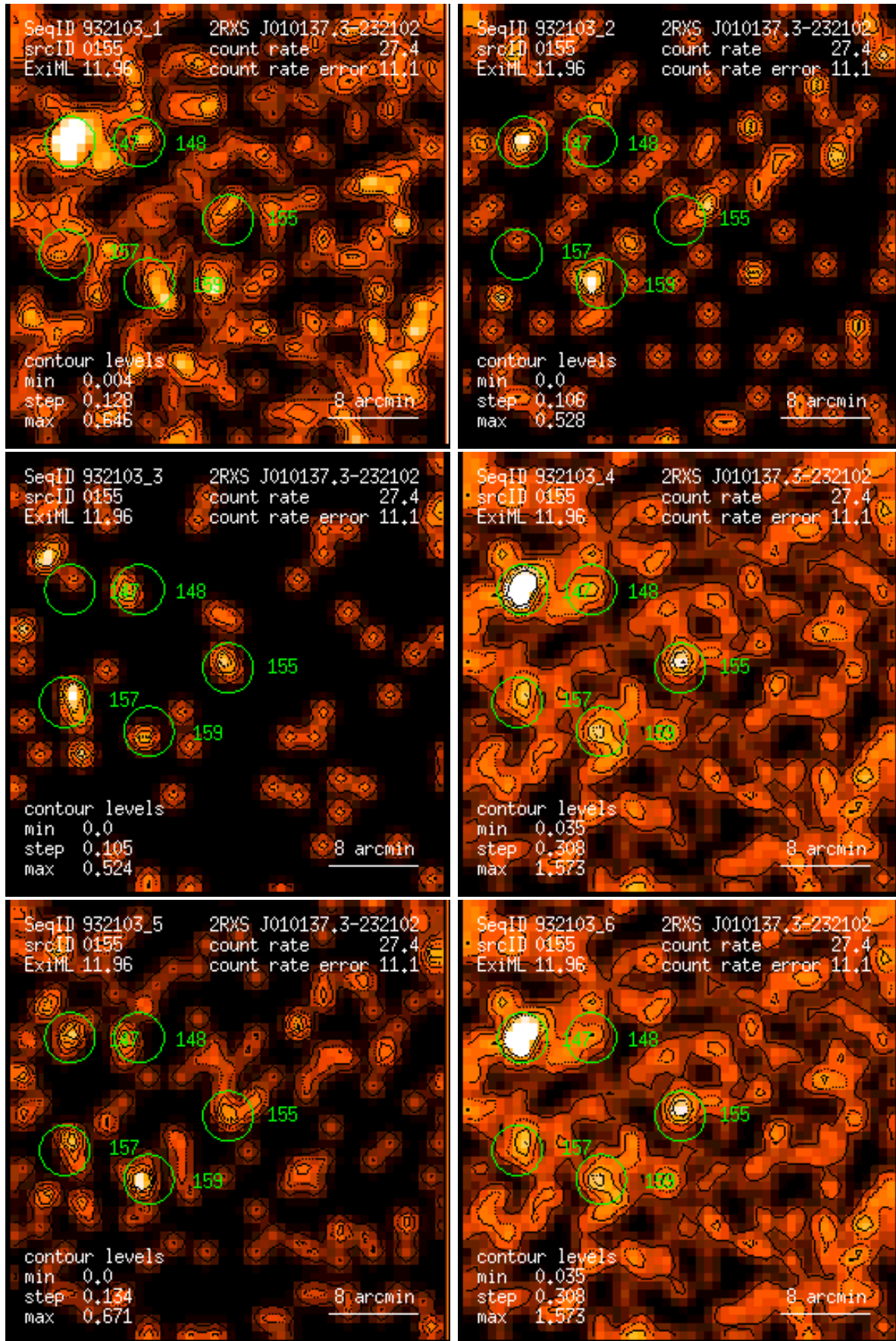
Figure 155: RASS 932103: detection 0155: band rate images, Gaussian filter: (1) PSPC channels 11 – 41, (2) 52 – 90, (3) 91 – 201, (4) 11 – 235, (5) 52 – 201, (6) 11 – 201. Broad band rates in counts/ks. Band rate contour levels in counts/ks/arcmin 2 .
