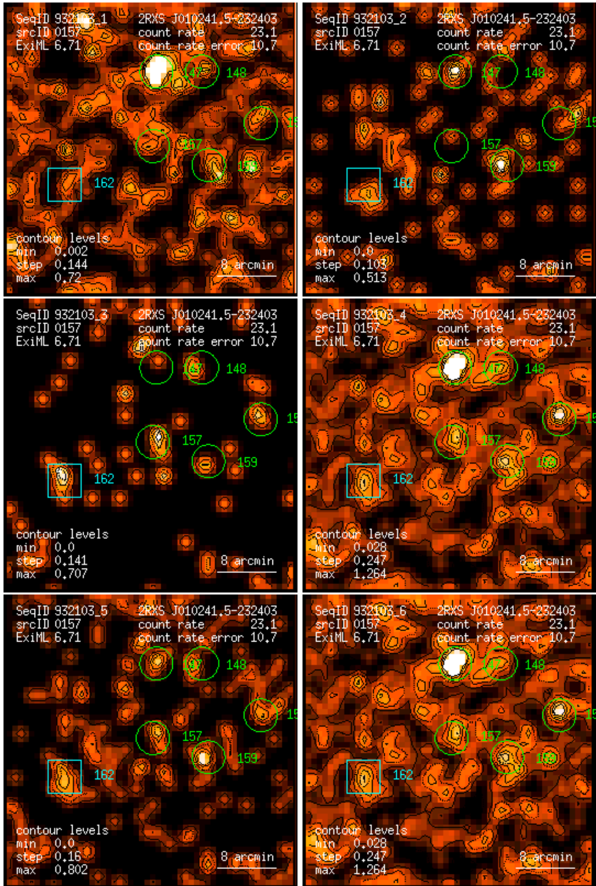
Figure 157: RASS 932103: detection 0157: band rate images, Gaussian filter: (1) PSPC channels 11 – 41, (2) 52 – 90, (3) 91 – 201, (4) 11 – 235, (5) 52 – 201, (6) 11 – 201. Broad band rates in counts/ks. Band rate contour levels in counts/ks/arcmin 2 .
