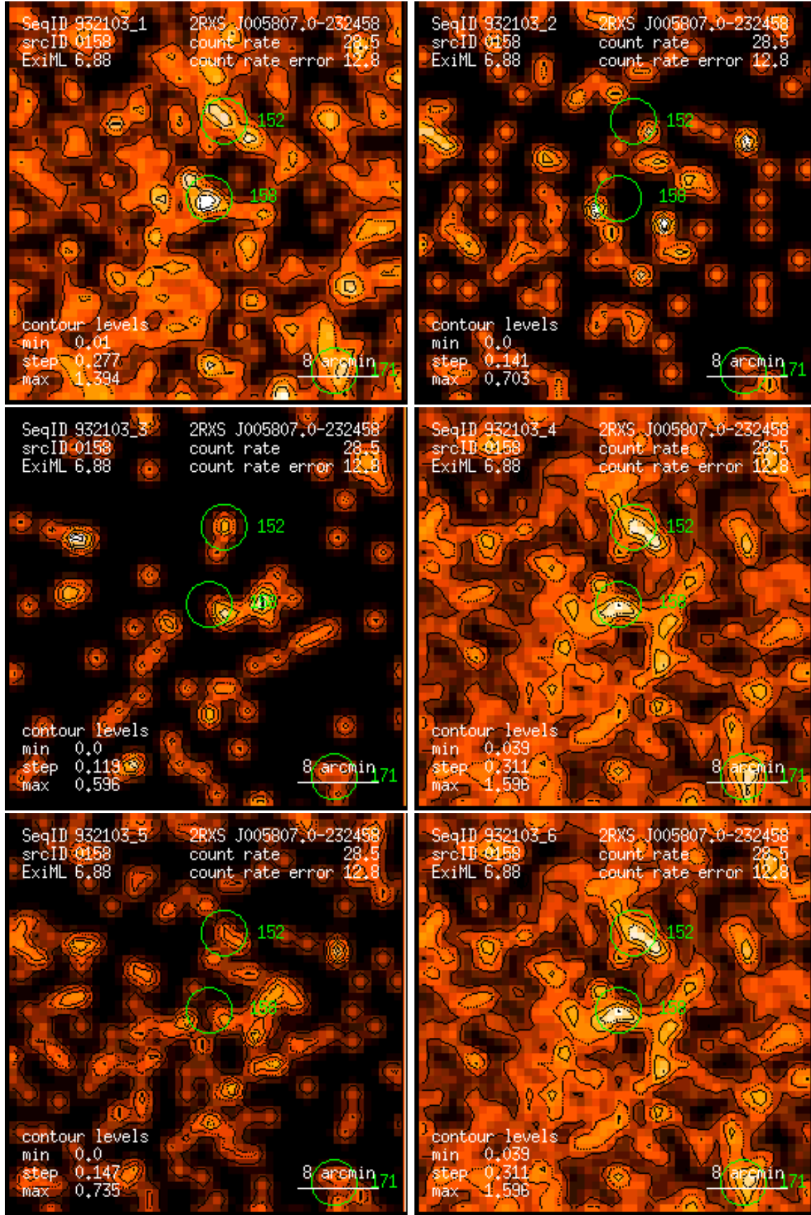
Figure 158: RASS 932103: detection 0158: band rate images, Gaussian filter: (1) PSPC channels 11 – 41, (2) 52 – 90, (3) 91 – 201, (4) 11 – 235, (5) 52 – 201, (6) 11 – 201. Broad band rates in counts/ks. Band rate contour levels in counts/ks/arcmin 2 .
