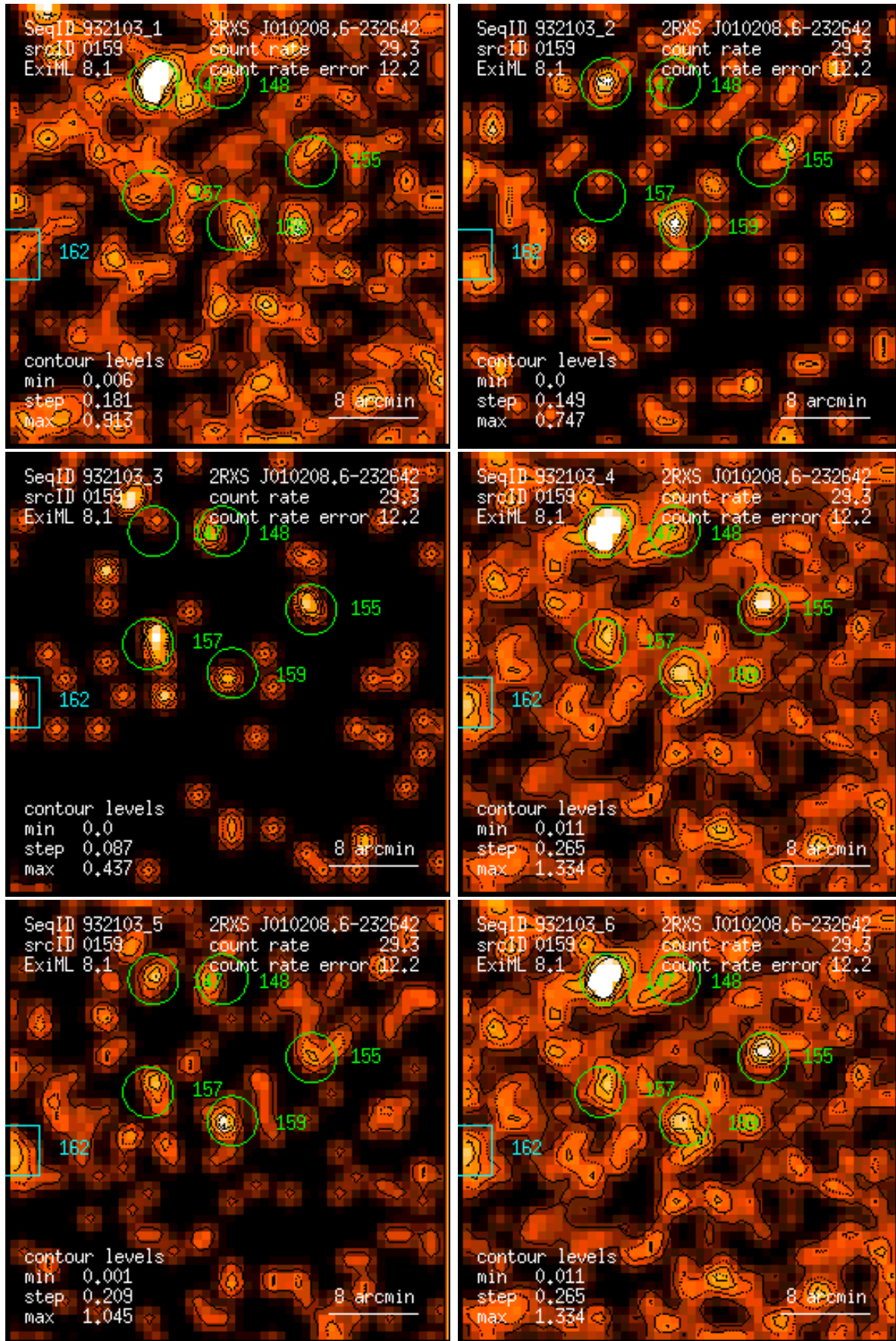
Figure 159: RASS 932103: detection 0159: band rate images, Gaussian filter: (1) PSPC channels 11 – 41, (2) 52 – 90, (3) 91 – 201, (4) 11 – 235, (5) 52 – 201, (6) 11 – 201. Broad band rates in counts/ks. Band rate contour levels in counts/ks/arcmin 2 .
