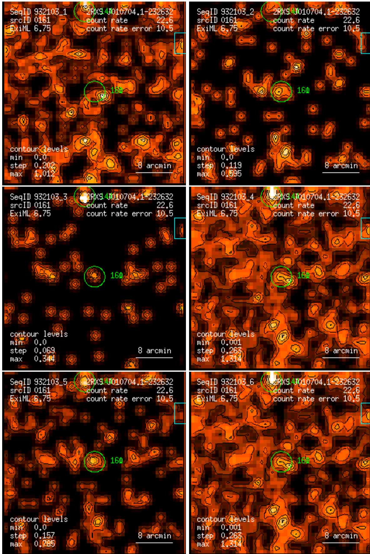
Figure 161: RASS 932103: detection 0161: band rate images, Gaussian filter: (1) PSPC channels 11 – 41, (2) 52 – 90, (3) 91 – 201, (4) 11 – 235, (5) 52 – 201, (6) 11 – 201. Broad band rates in counts/ks. Band rate contour levels in counts/ks/arcmin 2 .
