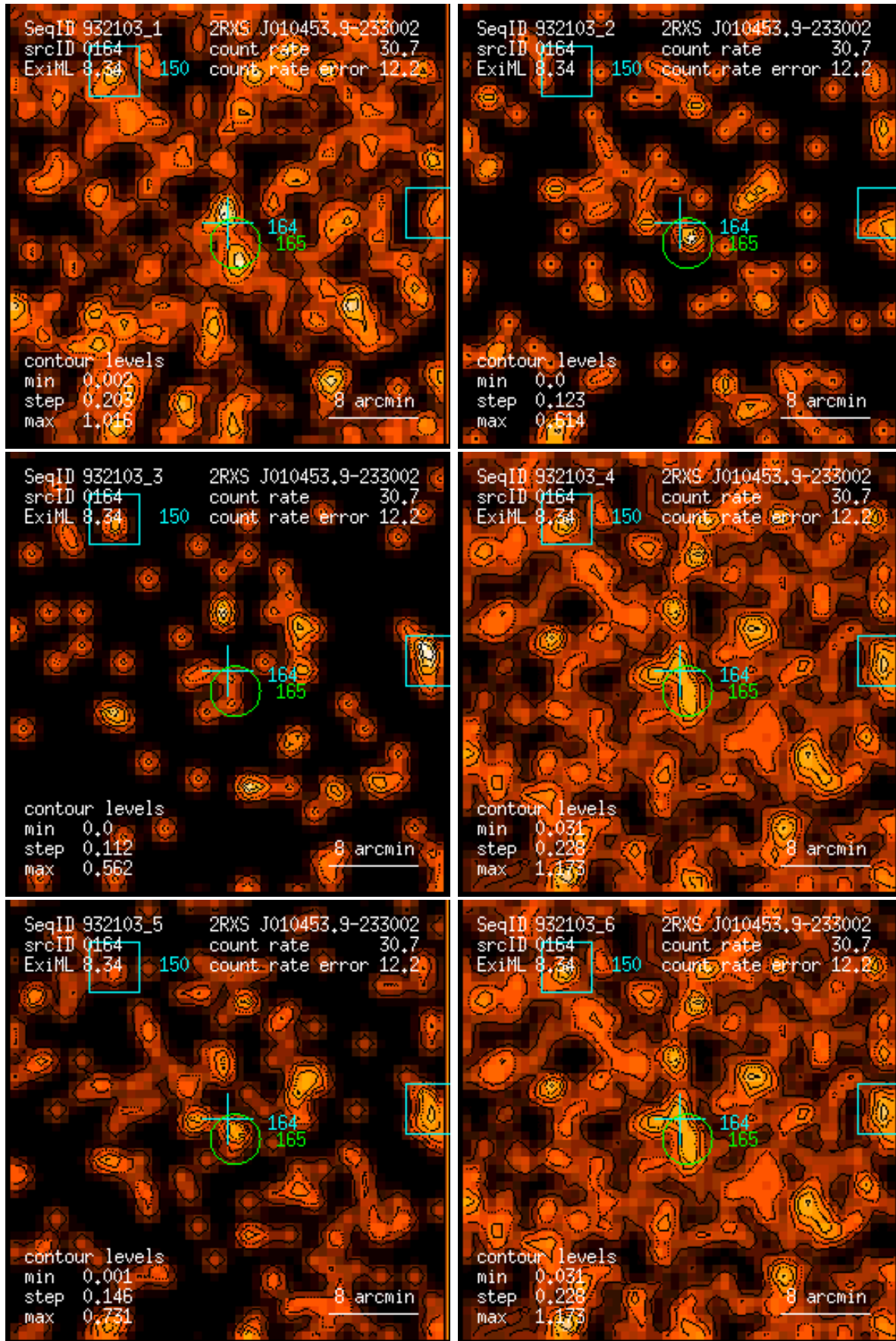
Figure 164: RASS 932103: detection 0164: band rate images, Gaussian filter: (1) PSPC channels 11 – 41, (2) 52 – 90, (3) 91 – 201, (4) 11 – 235, (5) 52 – 201, (6) 11 – 201. Broad band rates in counts/ks. Band rate contour levels in counts/ks/arcmin 2 .
