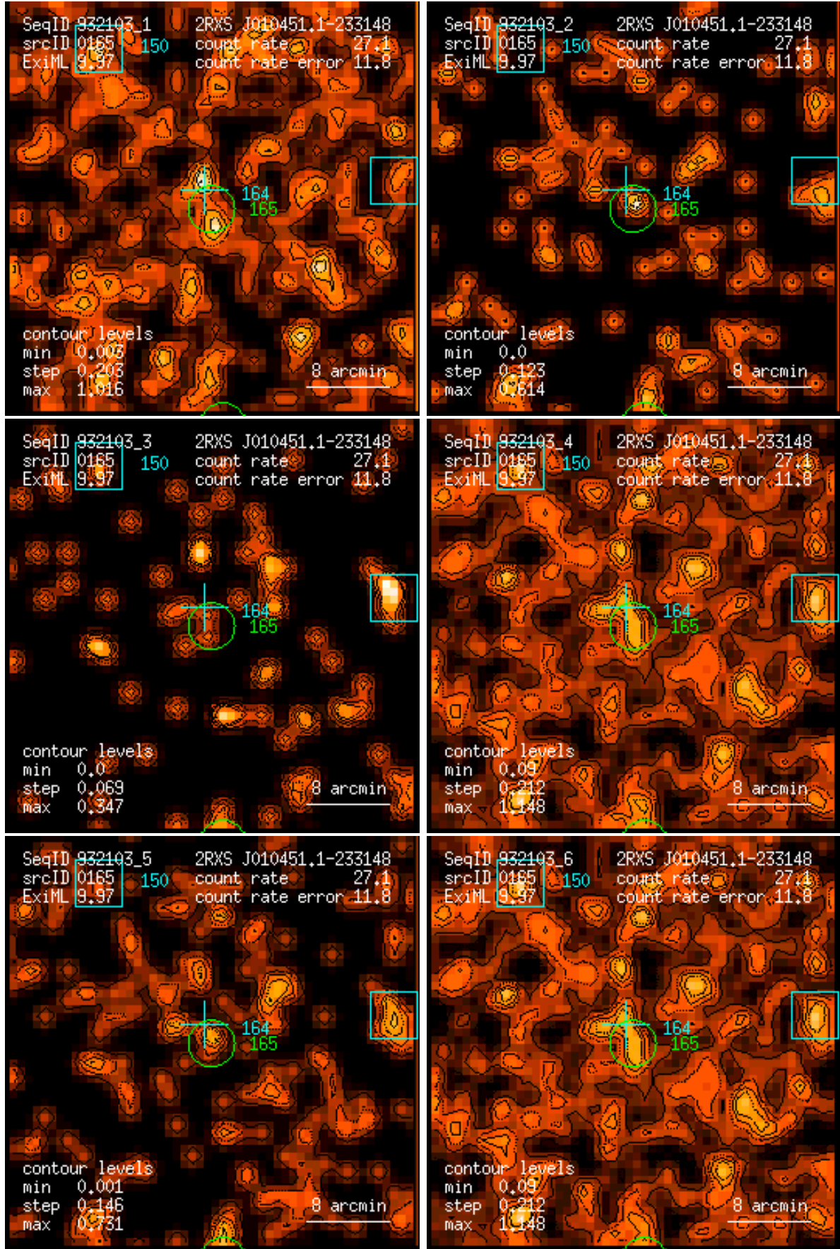
Figure 165: RASS 932103: detection 0165: band rate images, Gaussian filter: (1) PSPC channels 11 – 41, (2) 52 – 90, (3) 91 – 201, (4) 11 – 235, (5) 52 – 201, (6) 11 – 201. Broad band rates in counts/ks. Band rate contour levels in counts/ks/arcmin 2 .
