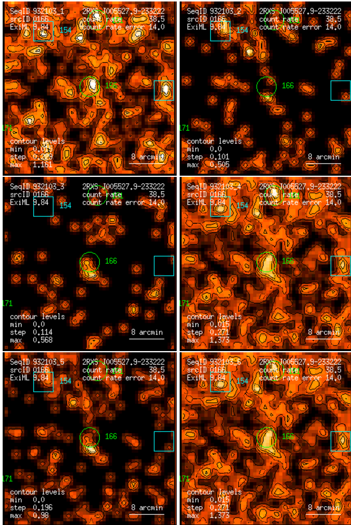
Figure 166: RASS 932103: detection 0166: band rate images, Gaussian filter: (1) PSPC channels 11 – 41, (2) 52 – 90, (3) 91 – 201, (4) 11 – 235, (5) 52 – 201, (6) 11 – 201. Broad band rates in counts/ks. Band rate contour levels in counts/ks/arcmin 2 .
