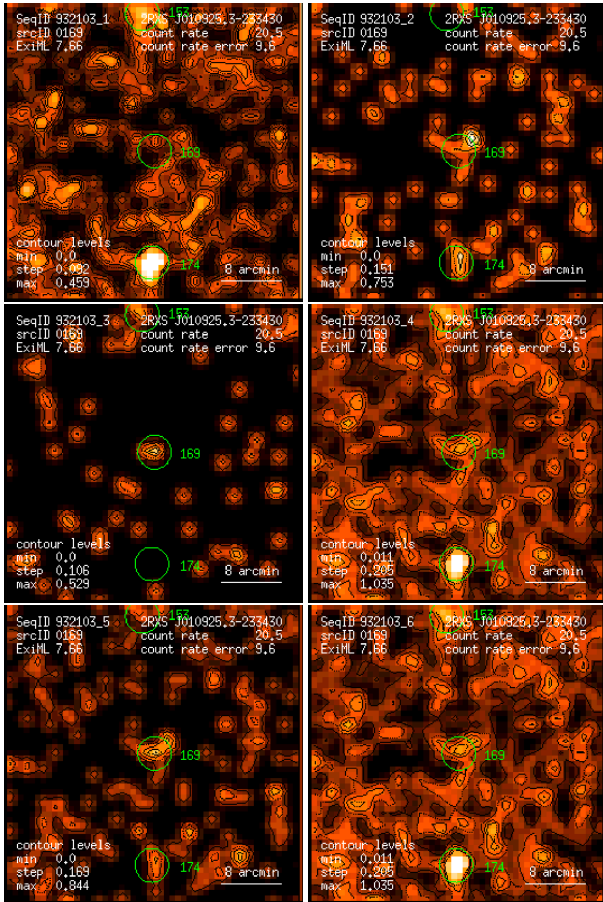
Figure 169: RASS 932103: detection 0169: band rate images, Gaussian filter: (1) PSPC channels 11 – 41, (2) 52 – 90, (3) 91 – 201, (4) 11 – 235, (5) 52 – 201, (6) 11 – 201. Broad band rates in counts/ks. Band rate contour levels in counts/ks/arcmin 2 .
