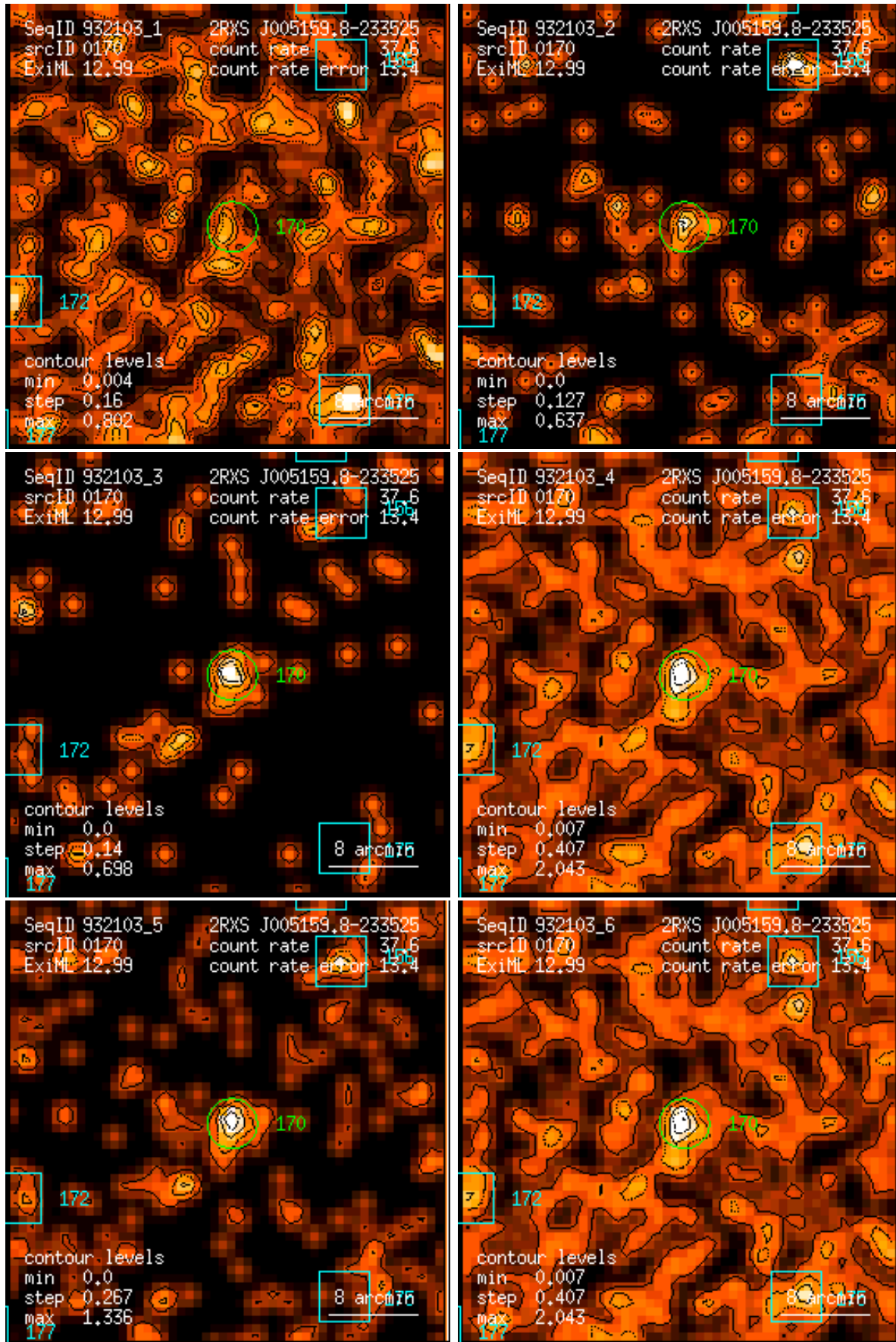
Figure 170: RASS 932103: detection 0170: band rate images, Gaussian filter: (1) PSPC channels 11 – 41, (2) 52 – 90, (3) 91 – 201, (4) 11 – 235, (5) 52 – 201, (6) 11 – 201. Broad band rates in counts/ks. Band rate contour levels in counts/ks/arcmin 2 .
