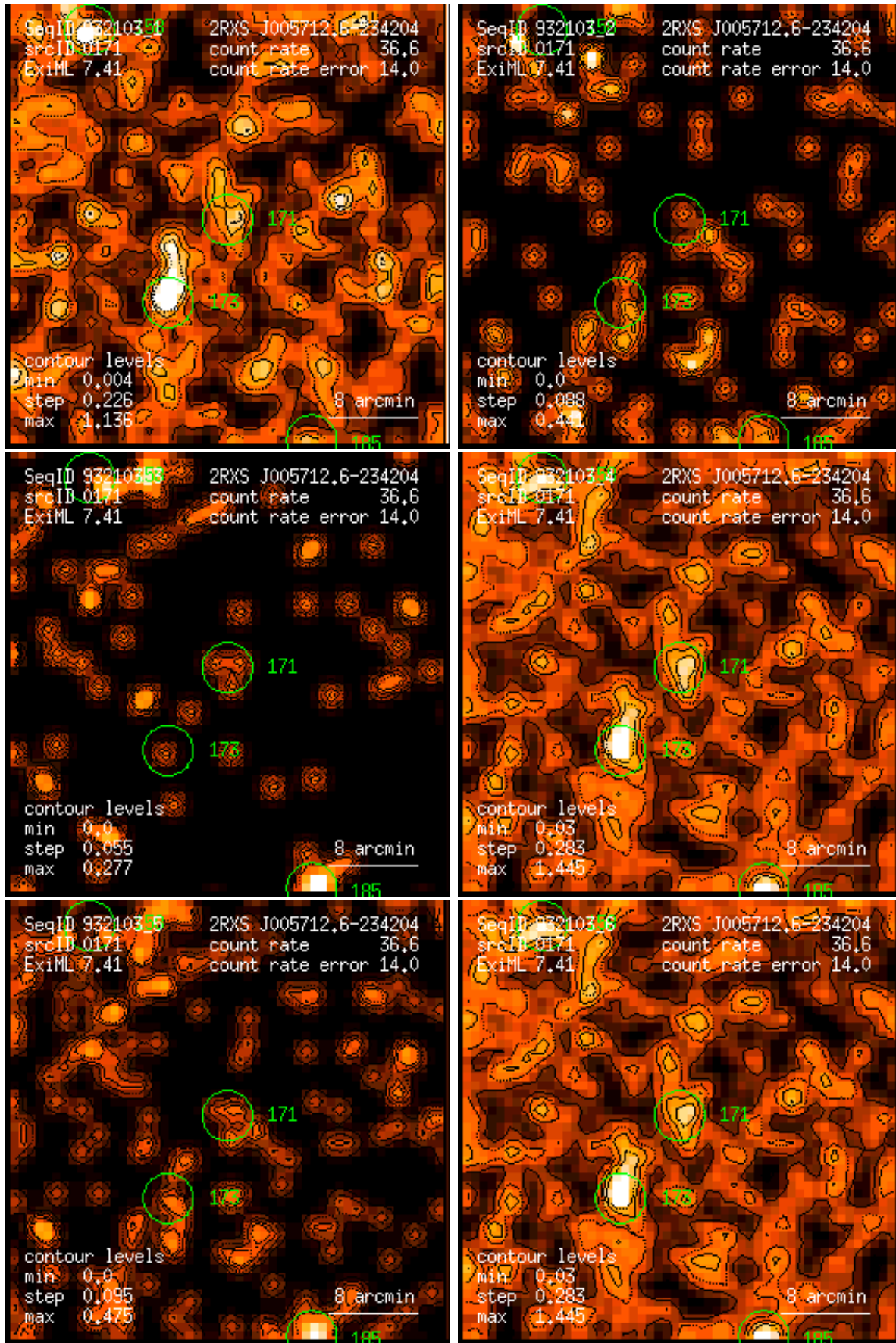
Figure 171: RASS 932103: detection 0171: band rate images, Gaussian filter: (1) PSPC channels 11 – 41, (2) 52 – 90, (3) 91 – 201, (4) 11 – 235, (5) 52 – 201, (6) 11 – 201. Broad band rates in counts/ks. Band rate contour levels in counts/ks/arcmin 2 .
