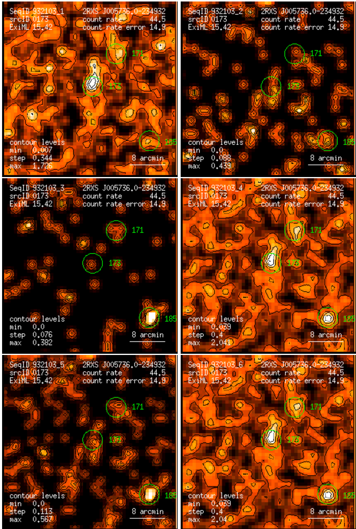
Figure 173: RASS 932103: detection 0173: band rate images, Gaussian filter: (1) PSPC channels 11 – 41, (2) 52 – 90, (3) 91 – 201, (4) 11 – 235, (5) 52 – 201, (6) 11 – 201. Broad band rates in counts/ks. Band rate contour levels in counts/ks/arcmin 2 .
