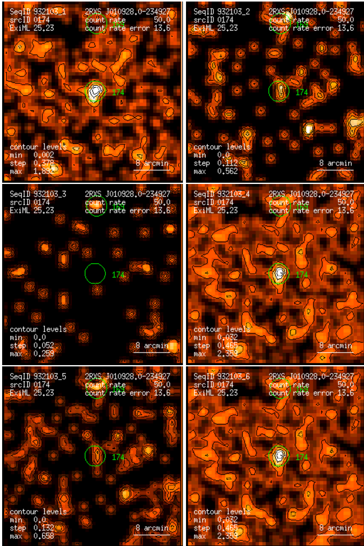
Figure 174: RASS 932103: detection 0174: band rate images, Gaussian filter: (1) PSPC channels 11 – 41, (2) 52 – 90, (3) 91 – 201, (4) 11 – 235, (5) 52 – 201, (6) 11 – 201. Broad band rates in counts/ks. Band rate contour levels in counts/ks/arcmin 2 .
