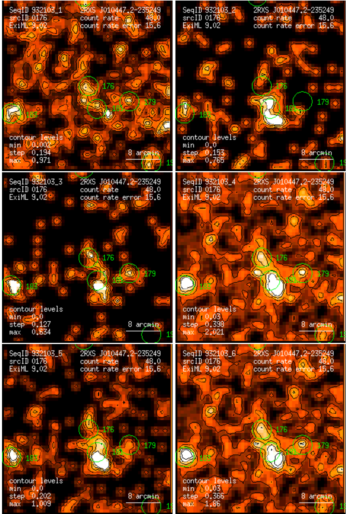
Figure 176: RASS 932103: detection 0176: band rate images, Gaussian filter: (1) PSPC channels 11 – 41, (2) 52 – 90, (3) 91 – 201, (4) 11 – 235, (5) 52 – 201, (6) 11 – 201. Broad band rates in counts/ks. Band rate contour levels in counts/ks/arcmin 2 .
