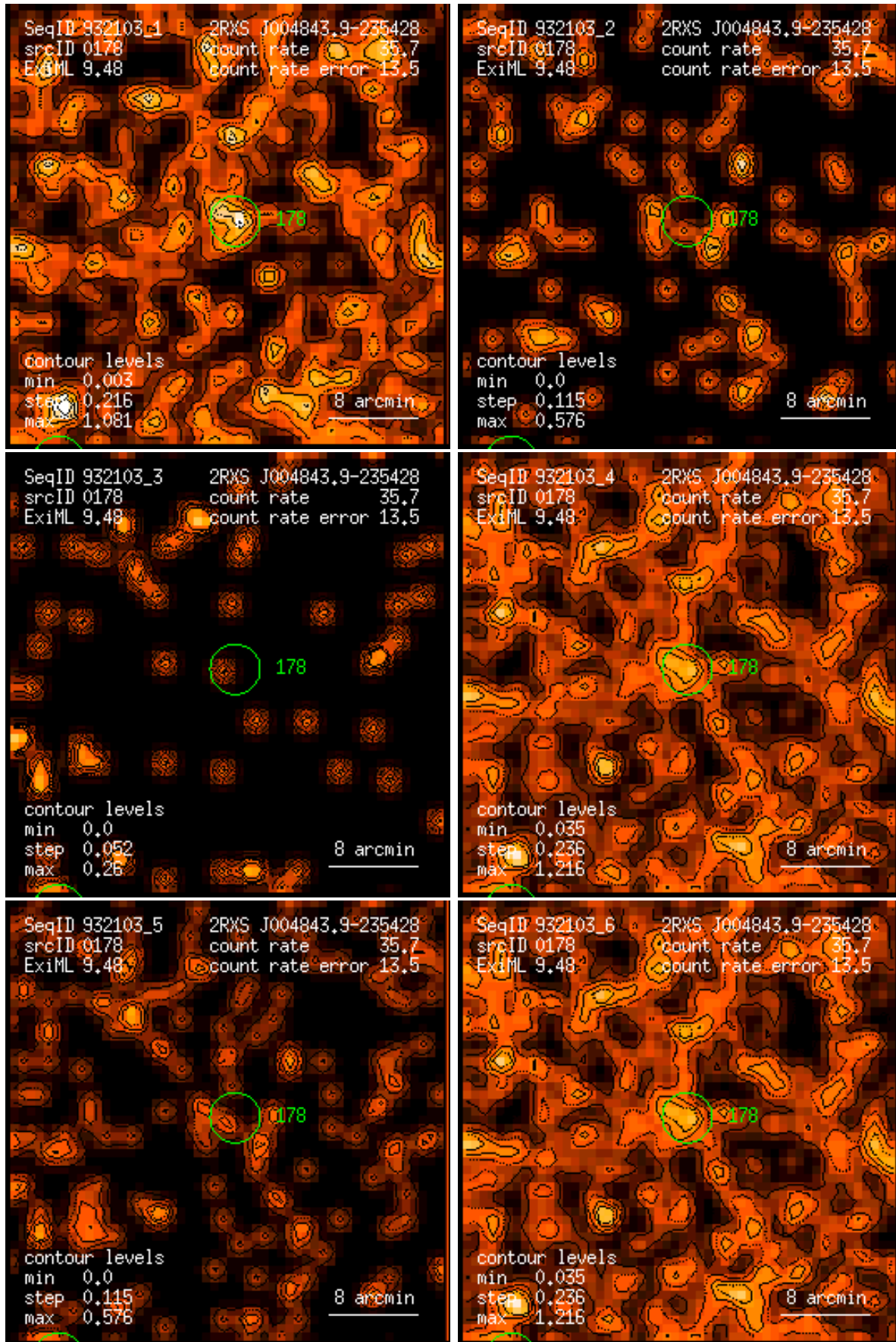
Figure 178: RASS 932103: detection 0178: band rate images, Gaussian filter: (1) PSPC channels 11 – 41, (2) 52 – 90, (3) 91 – 201, (4) 11 – 235, (5) 52 – 201, (6) 11 – 201. Broad band rates in counts/ks. Band rate contour levels in counts/ks/arcmin 2 .
