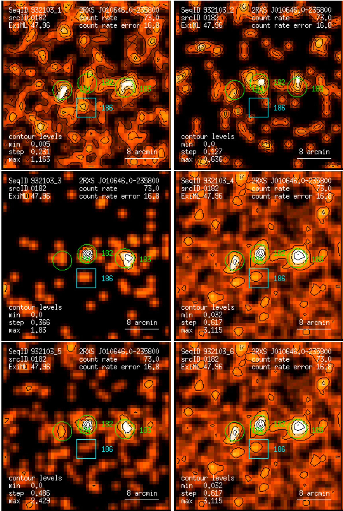
Figure 182: RASS 932103: detection 0182: band rate images, Gaussian filter: (1) PSPC channels 11 – 41, (2) 52 – 90, (3) 91 – 201, (4) 11 – 235, (5) 52 – 201, (6) 11 – 201. Broad band rates in counts/ks. Band rate contour levels in counts/ks/arcmin 2 .
