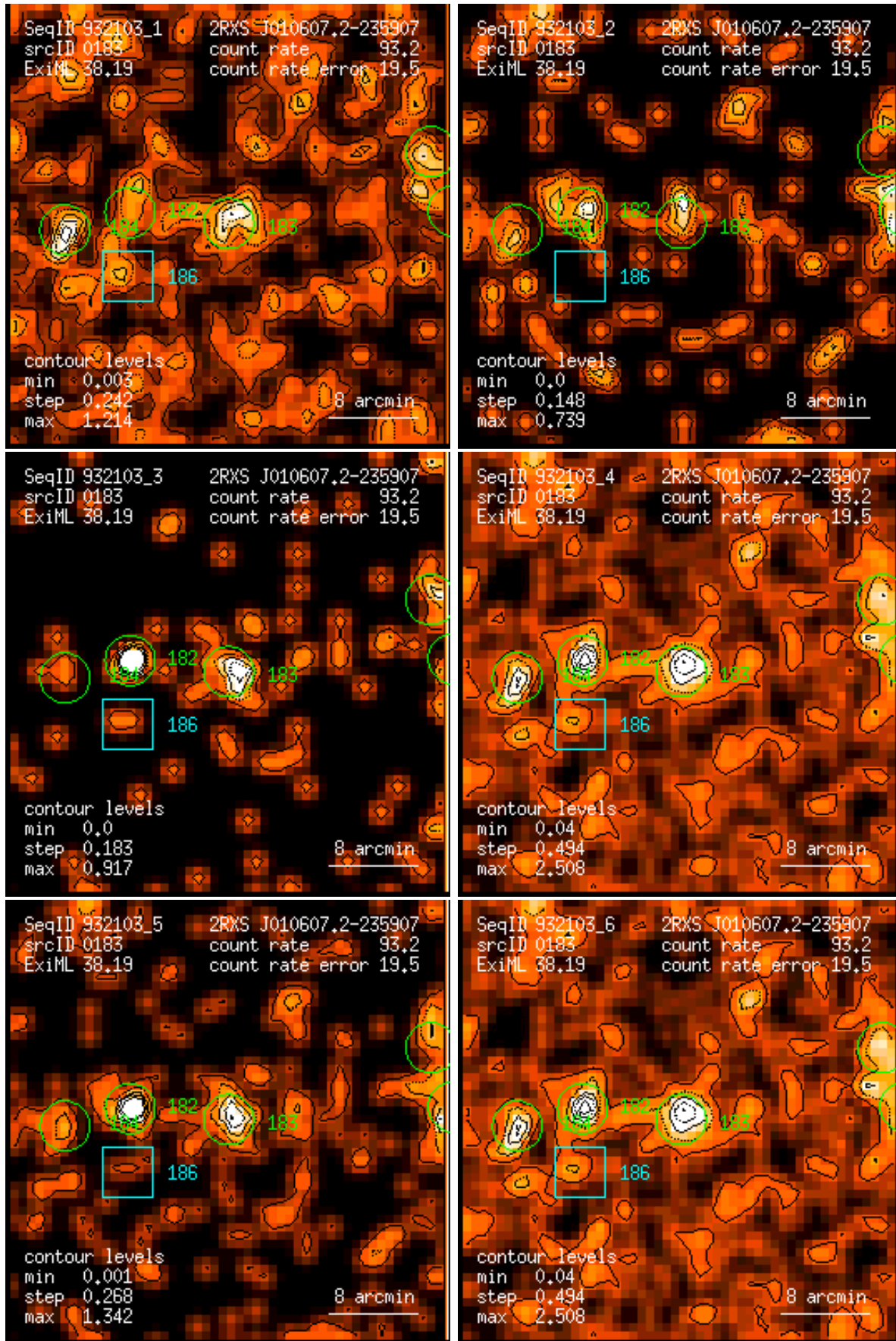
Figure 183: RASS 932103: detection 0183: band rate images, Gaussian filter: (1) PSPC channels 11 – 41, (2) 52 – 90, (3) 91 – 201, (4) 11 – 235, (5) 52 – 201, (6) 11 – 201. Broad band rates in counts/ks. Band rate contour levels in counts/ks/arcmin 2 .
