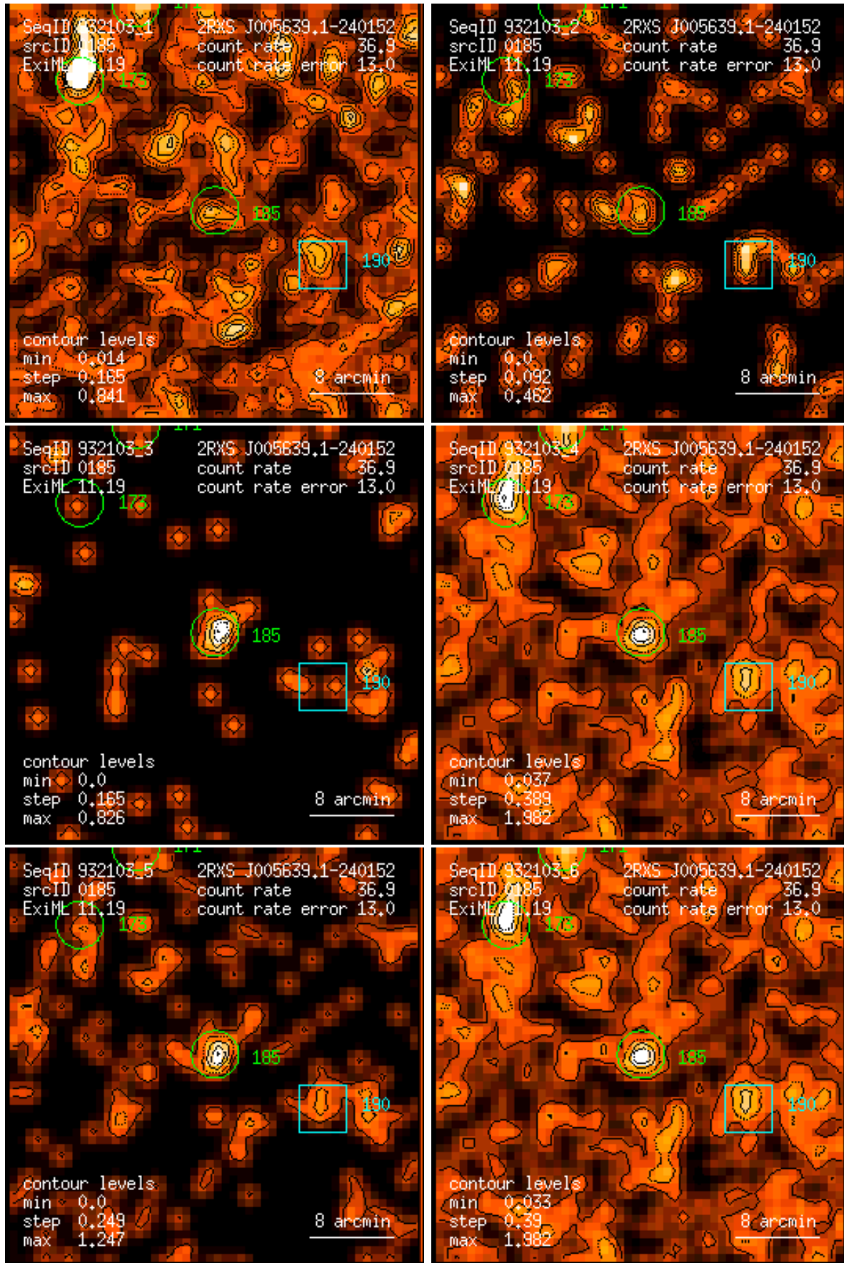
Figure 185: RASS 932103: detection 0185: band rate images, Gaussian filter: (1) PSPC channels 11 – 41, (2) 52 – 90, (3) 91 – 201, (4) 11 – 235, (5) 52 – 201, (6) 11 – 201. Broad band rates in counts/ks. Band rate contour levels in counts/ks/arcmin 2 .
