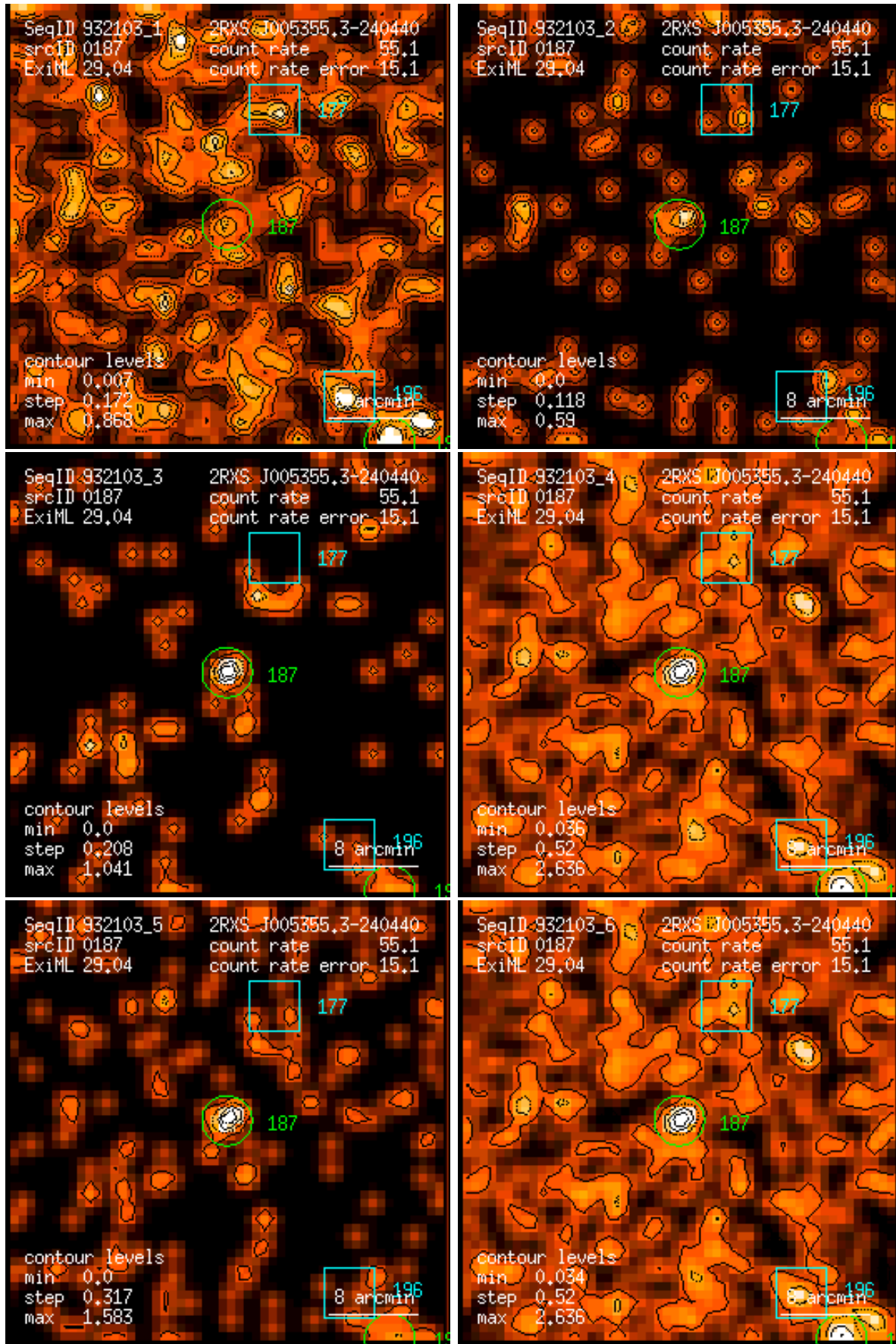
Figure 187: RASS 932103: detection 0187: band rate images, Gaussian filter: (1) PSPC channels 11 – 41, (2) 52 – 90, (3) 91 – 201, (4) 11 – 235, (5) 52 – 201, (6) 11 – 201. Broad band rates in counts/ks. Band rate contour levels in counts/ks/arcmin 2 .
