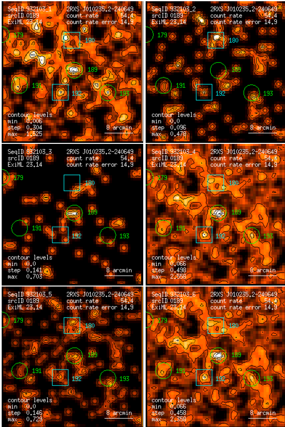
Figure 189: RASS 932103: detection 0189: band rate images, Gaussian filter: (1) PSPC channels 11 – 41, (2) 52 – 90, (3) 91 – 201, (4) 11 – 235, (5) 52 – 201, (6) 11 – 201. Broad band rates in counts/ks. Band rate contour levels in counts/ks/arcmin 2 .
