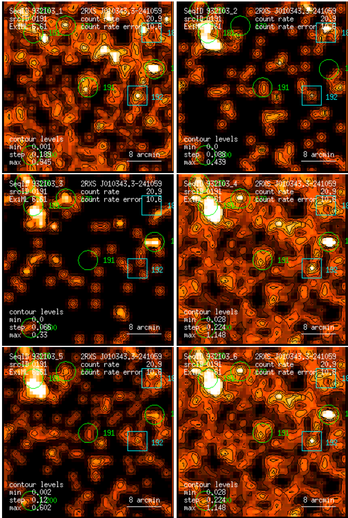
Figure 191: RASS 932103: detection 0191: band rate images, Gaussian filter: (1) PSPC channels 11 – 41, (2) 52 – 90, (3) 91 – 201, (4) 11 – 235, (5) 52 – 201, (6) 11 – 201. Broad band rates in counts/ks. Band rate contour levels in counts/ks/arcmin 2 .
