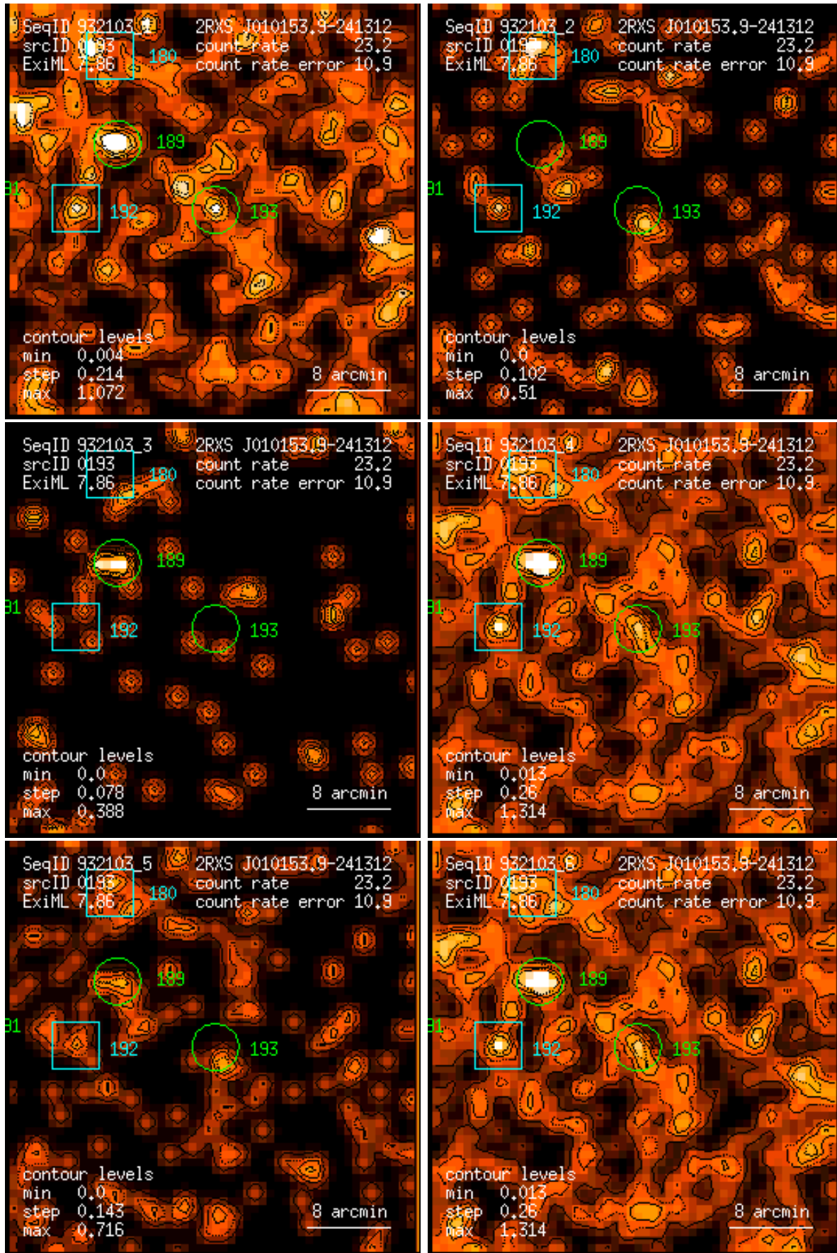
Figure 193: RASS 932103: detection 0193: band rate images, Gaussian filter: (1) PSPC channels 11 – 41, (2) 52 – 90, (3) 91 – 201, (4) 11 – 235, (5) 52 – 201, (6) 11 – 201. Broad band rates in counts/ks. Band rate contour levels in counts/ks/arcmin 2 .
