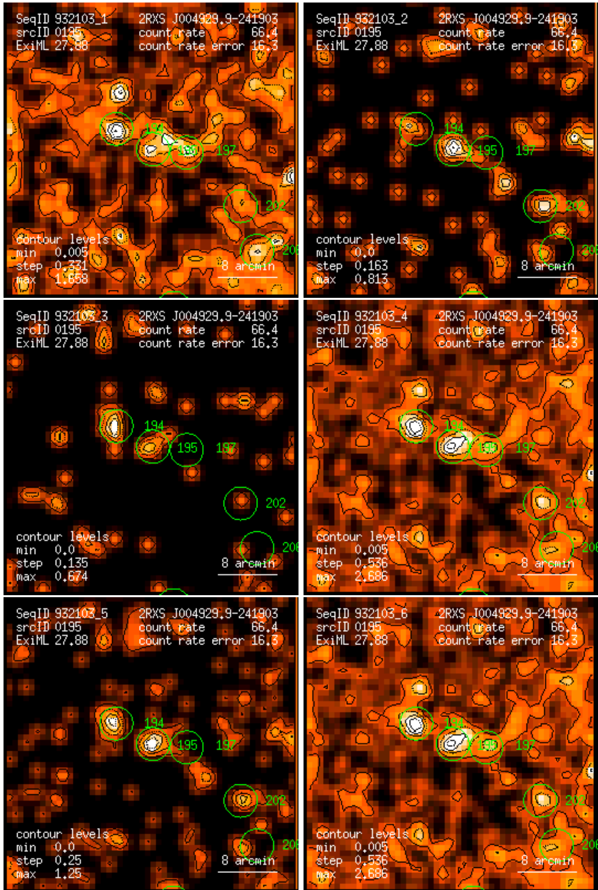
Figure 195: RASS 932103: detection 0195: band rate images, Gaussian filter: (1) PSPC channels 11 – 41, (2) 52 – 90, (3) 91 – 201, (4) 11 – 235, (5) 52 – 201, (6) 11 – 201. Broad band rates in counts/ks. Band rate contour levels in counts/ks/arcmin 2 .
