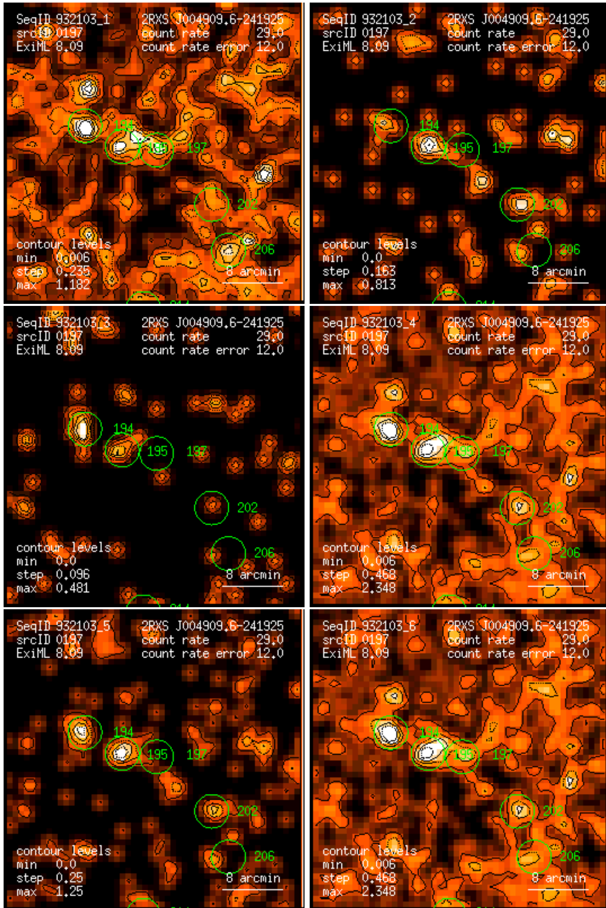
Figure 197: RASS 932103: detection 0197: band rate images, Gaussian filter: (1) PSPC channels 11 – 41, (2) 52 – 90, (3) 91 – 201, (4) 11 – 235, (5) 52 – 201, (6) 11 – 201. Broad band rates in counts/ks. Band rate contour levels in counts/ks/arcmin 2 .
