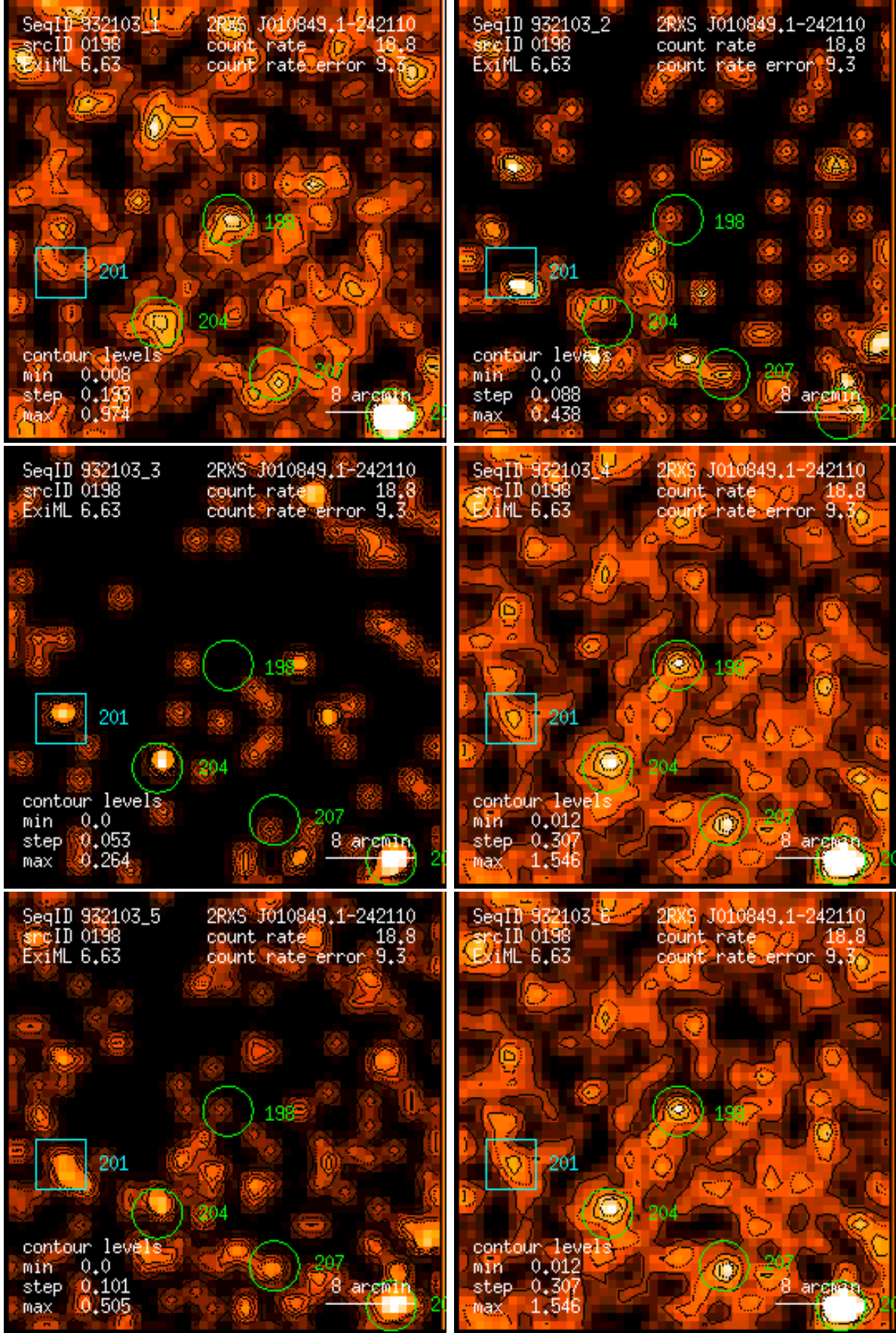
Figure 198: RASS 932103: detection 0198: band rate images, Gaussian filter: (1) PSPC channels 11 – 41, (2) 52 – 90, (3) 91 – 201, (4) 11 – 235, (5) 52 – 201, (6) 11 – 201. Broad band rates in counts/ks. Band rate contour levels in counts/ks/arcmin 2 .
