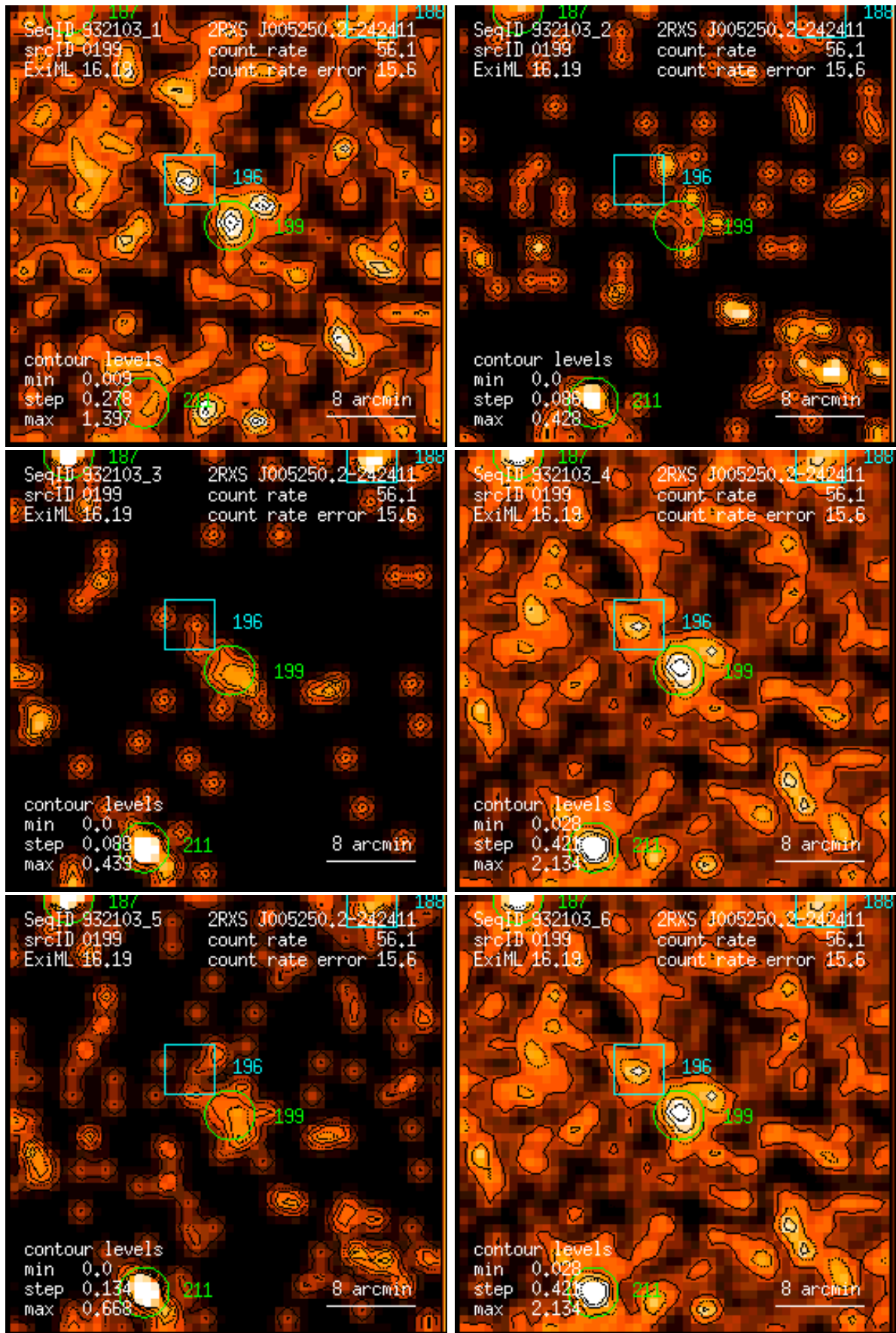
Figure 199: RASS 932103: detection 0199: band rate images, Gaussian filter: (1) PSPC channels 11 – 41, (2) 52 – 90, (3) 91 – 201, (4) 11 – 235, (5) 52 – 201, (6) 11 – 201. Broad band rates in counts/ks. Band rate contour levels in counts/ks/arcmin 2 .
