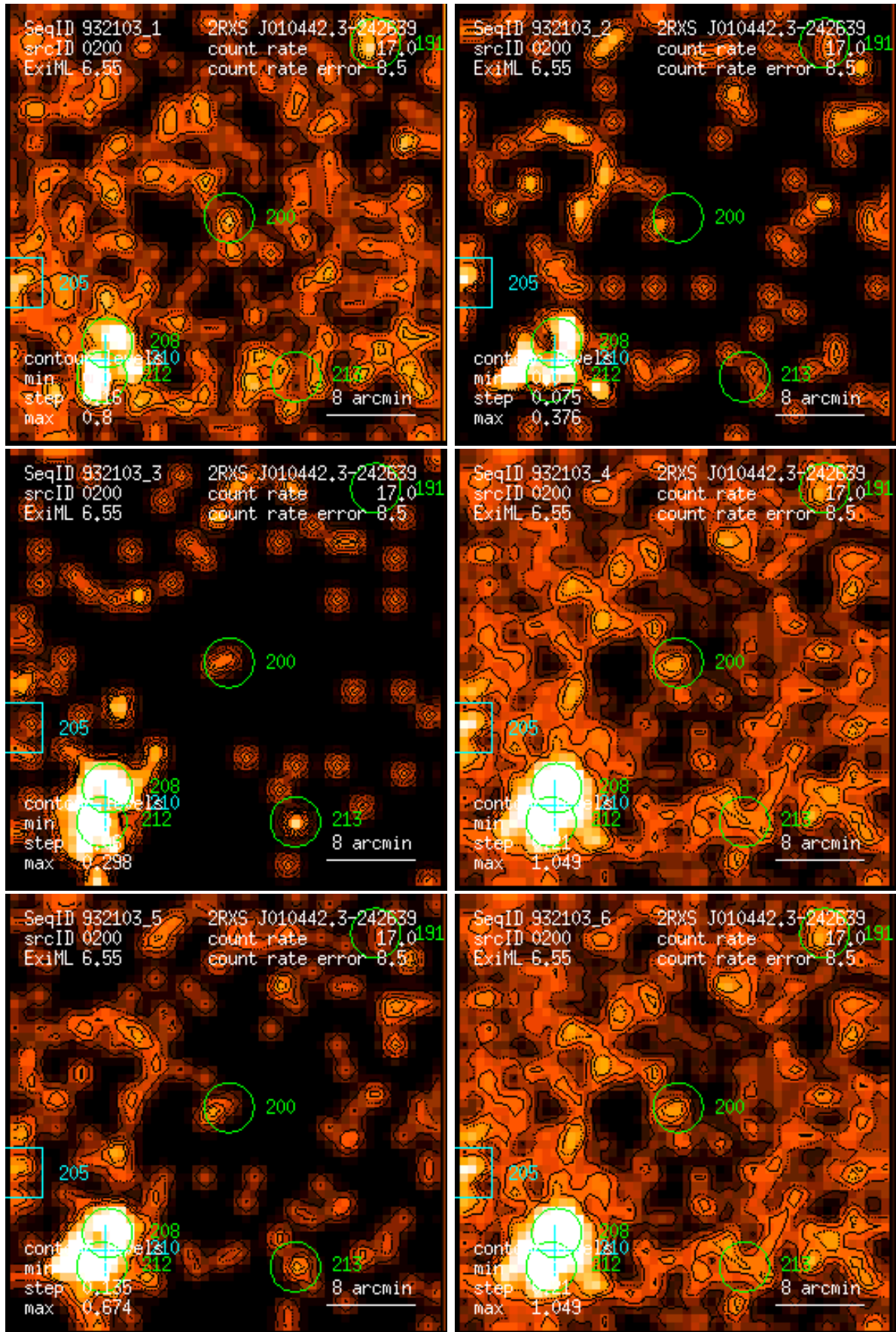
Figure 200: RASS 932103: detection 0200: band rate images, Gaussian filter: (1) PSPC channels 11 – 41, (2) 52 – 90, (3) 91 – 201, (4) 11 – 235, (5) 52 – 201, (6) 11 – 201. Broad band rates in counts/ks. Band rate contour levels in counts/ks/arcmin 2 .
