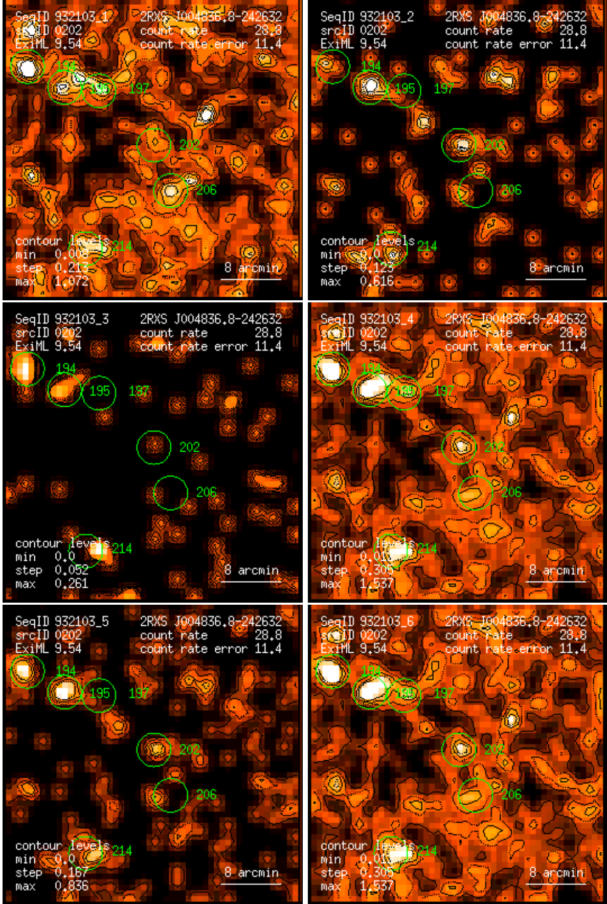
Figure 202: RASS 932103: detection 0202: band rate images, Gaussian filter: (1) PSPC channels 11 – 41, (2) 52 – 90, (3) 91 – 201, (4) 11 – 235, (5) 52 – 201, (6) 11 – 201. Broad band rates in counts/ks. Band rate contour levels in counts/ks/arcmin 2 .
