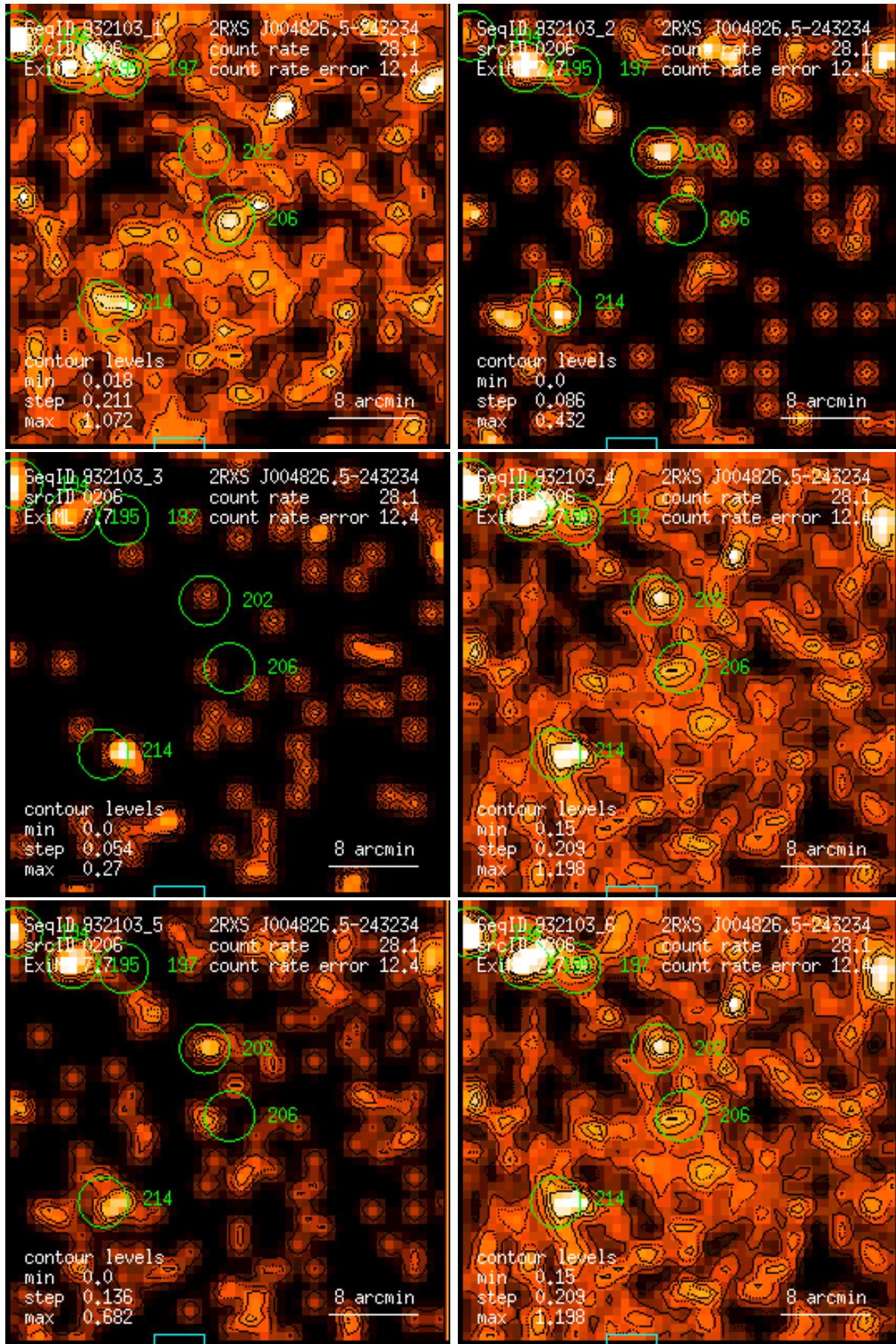
Figure 206: RASS 932103: detection 0206: band rate images, Gaussian filter: (1) PSPC channels 11 – 41, (2) 52 – 90, (3) 91 – 201, (4) 11 – 235, (5) 52 – 201, (6) 11 – 201. Broad band rates in counts/ks. Band rate contour levels in counts/ks/arcmin 2 .
