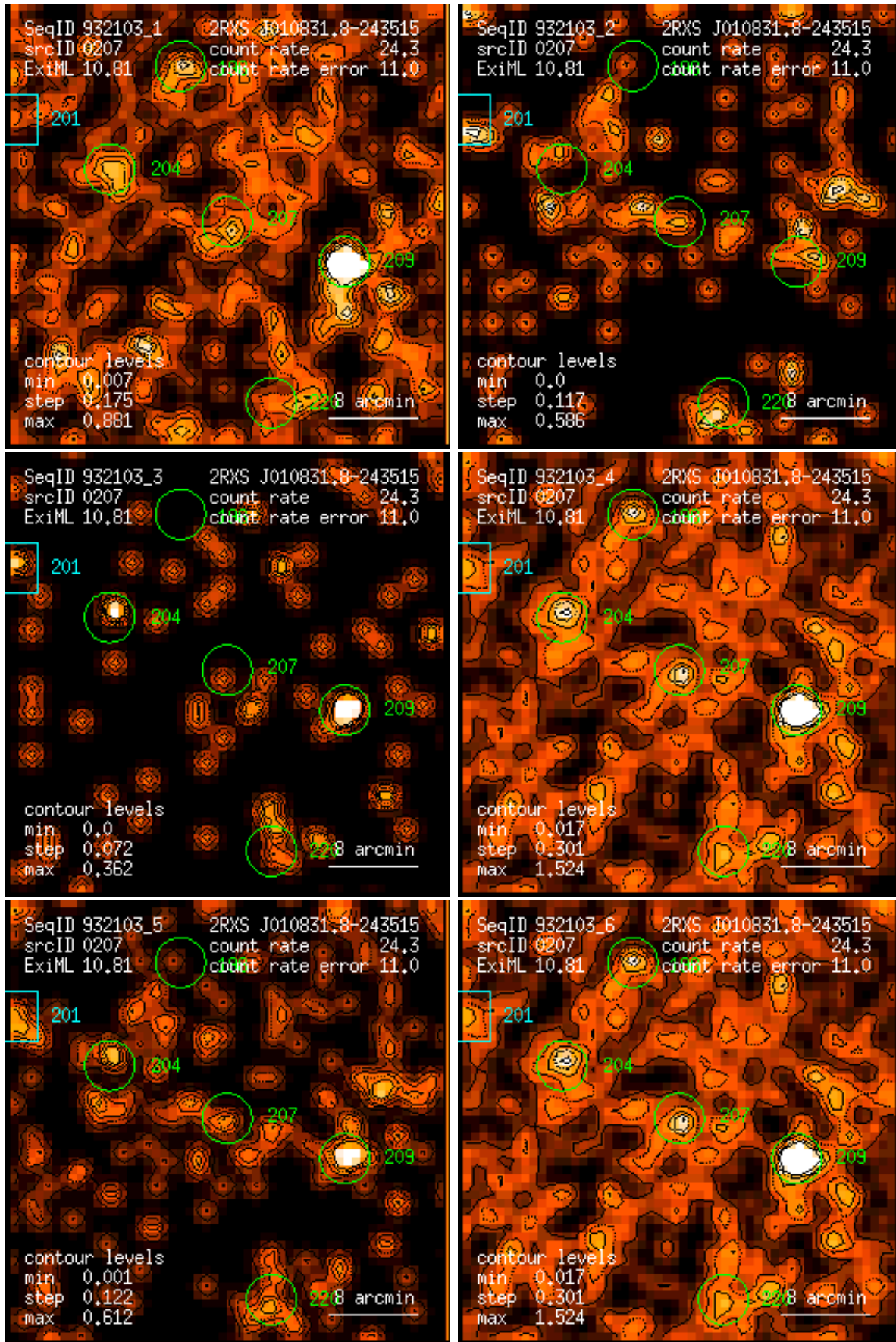
Figure 207: RASS 932103: detection 0207: band rate images, Gaussian filter: (1) PSPC channels 11 – 41, (2) 52 – 90, (3) 91 – 201, (4) 11 – 235, (5) 52 – 201, (6) 11 – 201. Broad band rates in counts/ks. Band rate contour levels in counts/ks/arcmin 2 .
