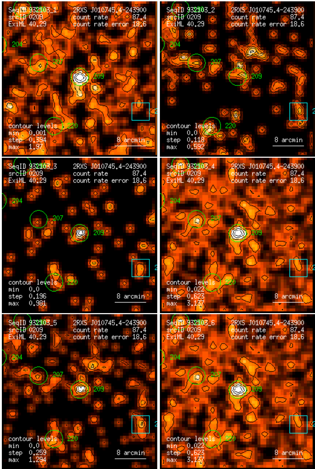
Figure 209: RASS 932103: detection 0209: band rate images, Gaussian filter: (1) PSPC channels 11 – 41, (2) 52 – 90, (3) 91 – 201, (4) 11 – 235, (5) 52 – 201, (6) 11 – 201. Broad band rates in counts/ks. Band rate contour levels in counts/ks/arcmin 2 .
